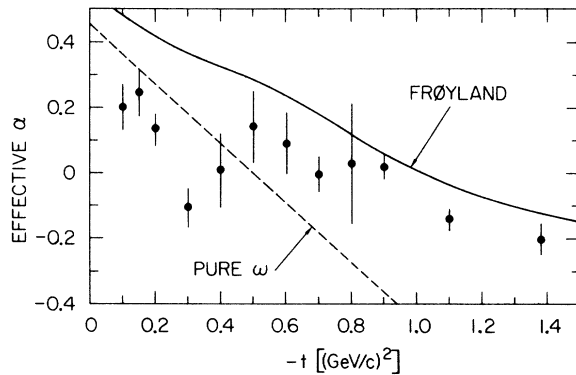
Fig. 4. Values of the effective \alpha are plotted versus |t| . The dashed line indicates the \alpha(t) expected for pure \omega exchange. The solid line is from the model of Frøyland.
