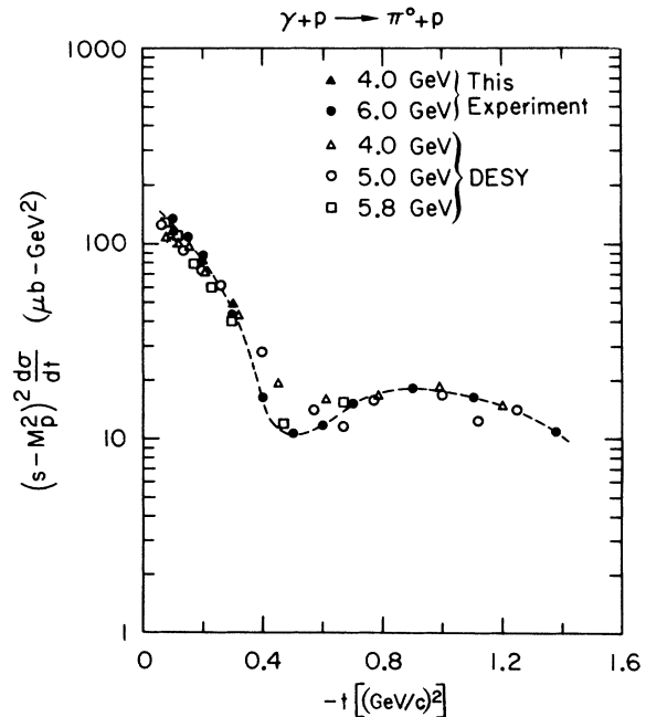
Fig. 7. Results from this experiment, expressed as (s - M_p^2)^2 d\sigma/dt in \mu\text{b-GeV}^2 , are plotted versus |t| together with measurements from DESY for comparison.
