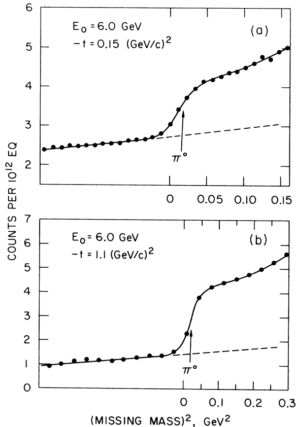
Fig. 2. The observed proton yield, in counts per hodoscope element per 10^{12} equivalent quanta (EQ), is plotted versus (\text{missing mass})^2 in the vicinity of the \pi^0 threshold. The photon end-point energy is 6 GeV, and t = -0.15 (GeV/c) 2 in (a) and -1.1 (GeV/c) 2 in (b).
