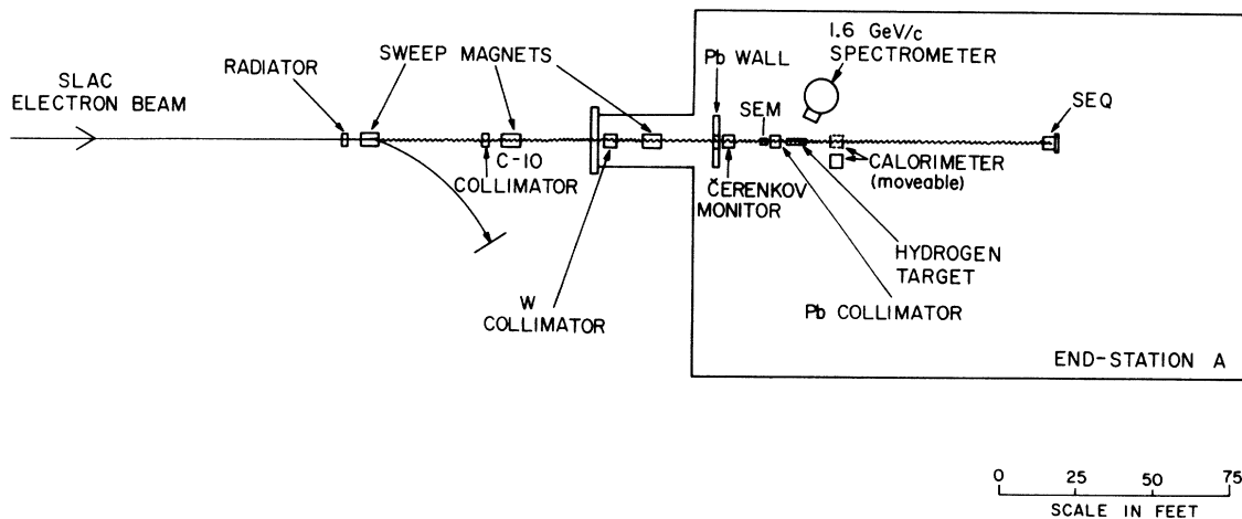
Fig. 1. Experimental arrangement for measurement of \pi^0 photoproduction cross sections.
