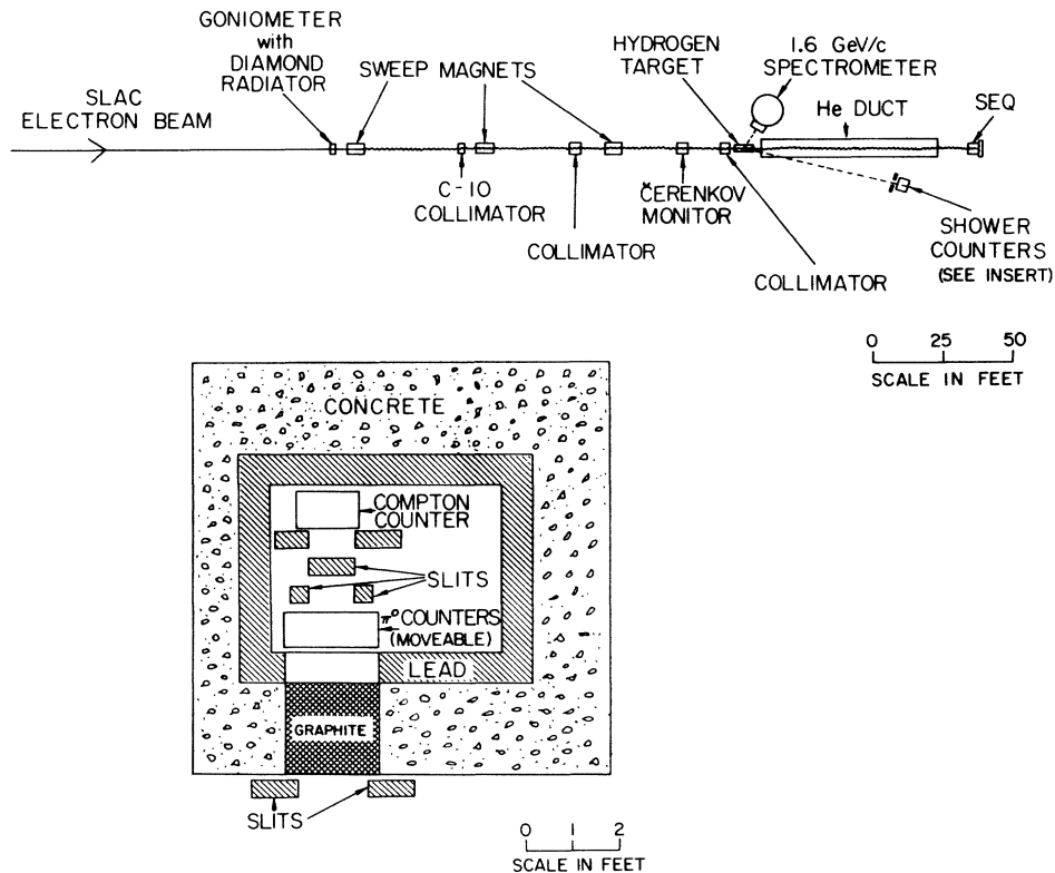
Fig. 8. Experimental arrangement for measurement of the asymmetry in \pi^0 photoproduction with polarized photons.
