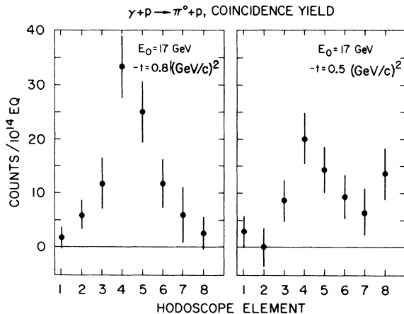
Fig. 6. Shown are proton yields in the hodoscope, in coincidence with \pi^0 -decay photons in a shower counter. The units are counts per hodoscope element per 10^{14} equivalent quanta (EQ), plotted versus hodoscope number. The average photon energy is 17 GeV and two momentum transfers are represented: t = -0.8 (\text{GeV}/c)^2 and t = -0.5 (\text{GeV}/c)^2 .
