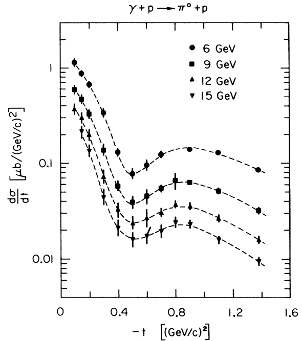
Fig. 5. d\sigma/dt in \mu\text{b}/(\text{GeV}/c)^2 is plotted versus |t| for incident photon energies of 6, 9, 12, and 15 GeV. The dashed lines are only to guide the eye.
