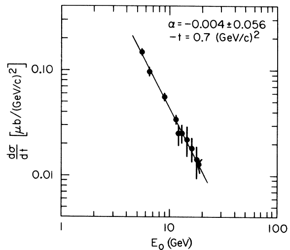
Fig. 3. For t = -0.7 (GeV/c) 2 , d\sigma/dt in \mu\text{b}/(\text{GeV}/c)^2 is plotted versus photon energy in GeV, with both scales logarithmic. The solid line is a fit of the form d\sigma/dt \sim E_0^{2\alpha - 2} \sim (s - M_p^2)^{2\alpha - 2} and the value of \alpha is shown.
