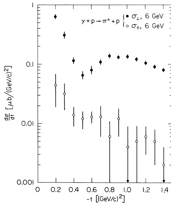
Fig. 12. Contributions to the \pi^0 photoproduction cross section for 6-GeV photons polarized normal to and parallel to the reaction plane, have been plotted separately in \mu\text{b}/(\text{GeV}/c)^2 versus |t| in (\text{GeV}/c)^2 .
