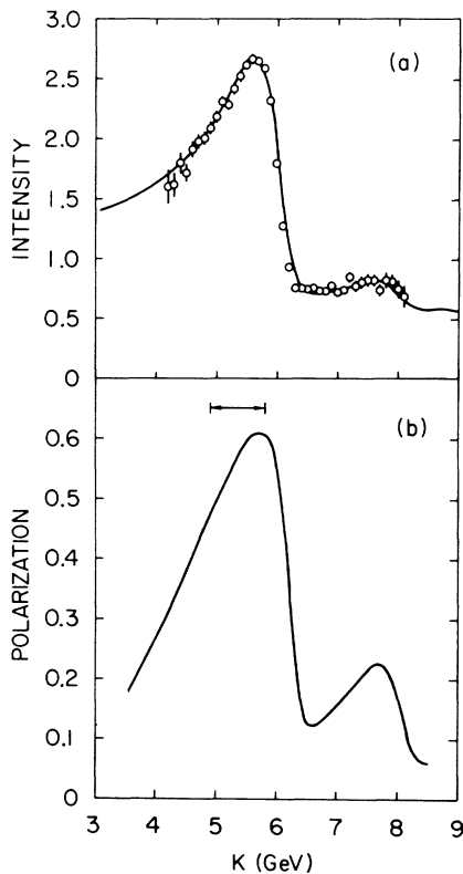
Fig. 9. (a) Shown is the intensity spectrum of coherent bremsstrahlung from the diamond used in this experiment, as measured by the SLAC pair spectrometer. The points were taken with the diamond oriented to give photons polarized normal to the reaction plane. The solid curve is a theoretical spectrum fitted to the measurements with polarization parallel to the reaction plane. (b) The solid curve shows the beam polarization corresponding to the computed spectrum in (a).
