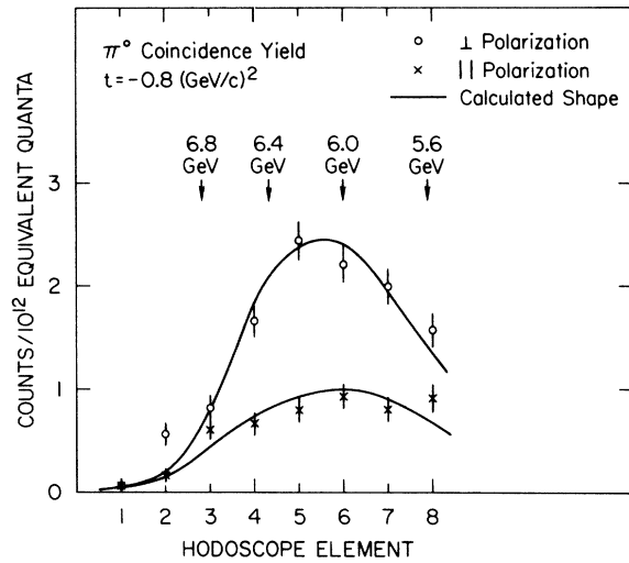
Fig. 10. Spectrometer shower-counter coincidence yields from a coherent bremsstrahlung beam are plotted versus hodoscope number. The spectrometer was set for t = -0.8 \text{ (GeV/c)}^2 , and the edge of the coherent spike in the beam was set at 6.74 GeV with an incident electron energy of 12 GeV. The photon energy variation across the hodoscope is indicated by the arrows.
