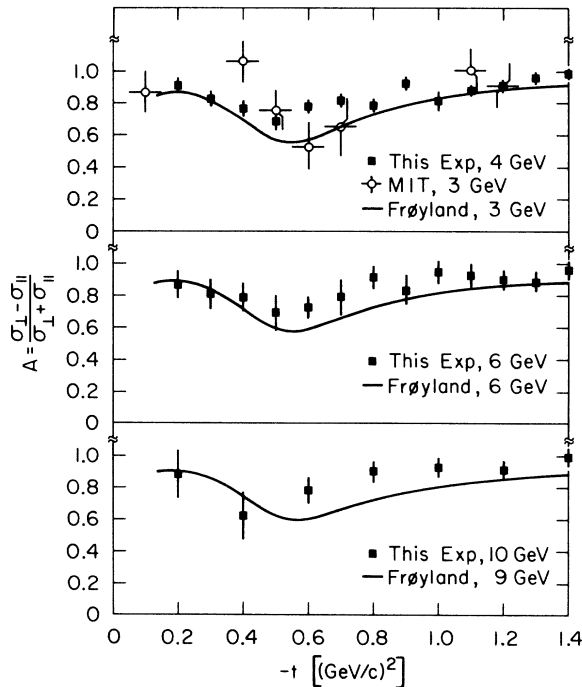
Fig. 11. The measured asymmetry at 4-, 6-, and 10-GeV average photon energies is plotted versus |t| . Measurements at 3 GeV by the MIT group are included for comparison. The solid curves are a theoretical prediction by Frøylund.
