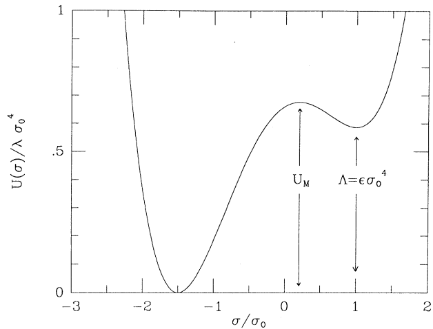
FIG. 1. The zero-temperature potential for nondegenerate vacua. \epsilon , the asymmetry parameter, is in general a function of temperature and of different couplings in the model.
