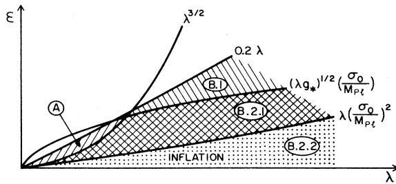
FIG. 2. Schematic display of all four possible scenarios for different values of the asymmetry parameter \epsilon . In case A the walls disappear in a time scale much smaller than the cosmological time scale t_G . In case B.1 the walls disappear in a time scale comparable to t_G . In case B.2.1 there can be one straight wall in a horizon volume but the walls disappear before dominating the energy density of the Universe. In case B.2.2 the walls dominate the energy density, causing a power-law inflation until they disappear.
