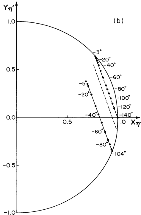
FIG. 3. Solutions for mixing parameters Y_{\eta'} and X_{\eta'} for the cases \Gamma(\iota \rightarrow 2\gamma) = 2.2 keV, 1.1 keV, and 0 as solid line, dot-dashed, and dashed lines, respectively. (a) corresponds to the (+) branch in Eq. (5.13) and (b) to the (-) branch.
