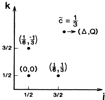
FIG. 1. Operator content of the \bar{c} = \frac{1}{3} minimal system (NS sector) (the first entry is the dimension of an operator and the second its change). Circles represent operators belonging to the R sector. The solid circles indicate the N=2 subsystem of \bar{c} = \frac{1}{3} .
