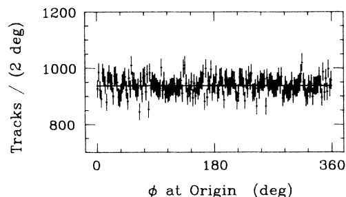
FIG. 2. Distribution in production azimuth for e^+ and e^- tracks from Bhabha scattering. The distribution is expected to be flat for a uniform tracking system and unpolarized e^+e^- colliding beams.
