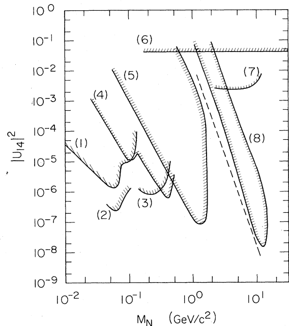
FIG. 1. Limits on |U_{14}|^2 as a function of neutrino mass M_N , as obtained from (1) TRIUMF \pi \rightarrow e\nu , Ref. 6; (2) SIN \pi \rightarrow e\nu , Ref. 7; (3) KEK K \rightarrow e\nu , Ref. 8; (4) CHARM experiment at CERN with a wide-band beam, Ref. 9; (5) CHARM experiment at CERN searching for D \rightarrow eN in a beam dump, Ref. 10; (6) universality, Ref. 16; (7) combined monojet searches at PEP, Refs. 12, 13, and 14; (8) secondary-vertex search in e^+e^- \rightarrow N\bar{N} at PEP, Ref. 18. The dashed line corresponds to \gamma c\tau of one meter for a fourth-generation neutrino produced in e^+e^- \rightarrow N\bar{N} at \sqrt{s} = 29 \text{ GeV} .
