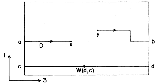
FIG. 2. Position of the string D connecting x and y in a periodic volume and the Polyakov loop W(d,c) . The points x and y are allowed to have an offset in the 2 and 4 directions as well.
