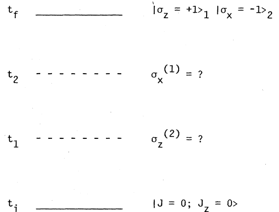
FIG. 4. A measurement of \sigma_z^{(2)} or \sigma_x^{(1)} is carried out in the interval between t_i and t_f . A measurement of \sigma_z^{(2)} at t_1 is certain to yield \sigma_z^{(2)}(t_1) = -1 ; a measurement of \sigma_x^{(1)} at t_2 is certain to yield \sigma_x^{(1)}(t_2) = +1 .
