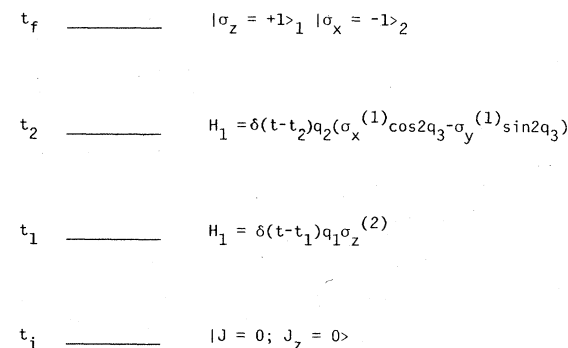
FIG. 5. Compensating measurements are carried out on two spin-correlated particles at t_1 and t_2 . After the measurements have been completed, it will be found that \Delta\Pi_2 = \sigma_x^{(2)}(t_f) = -1 and that \Delta\Pi_1 + \Delta\Pi_3 = \sigma_z^{(1)}(t_f) = +1 .
