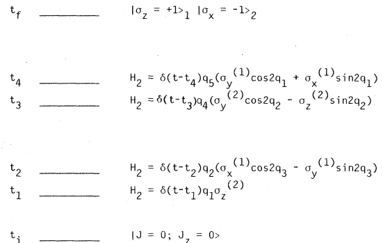
FIG. 6. Compensating measurements are performed on a two-particle system in such a way as to relate (\Delta\Pi_1 + \Delta\Pi_3) and \Delta\Pi_2 to the final state of the system and (\Delta\Pi_4 + \Delta\Pi_5) to its initial state. The initial conditions on the measuring devices are that q_{10} - q_{30} = \Pi_{10} + \Pi_{30} = q_{40} - q_{50} = \Pi_{40} + \Pi_{50} = 0 . After all measurements have been completed, it will be found that \Delta\Pi_1 + \Delta\Pi_3 = \sigma_z^{(1)}(t_f) = +1 , \Delta\Pi_2 = \sigma_x^{(2)}(t_f) = -1 , and \Delta\Pi_4 + \Delta\Pi_5 = 0 .
