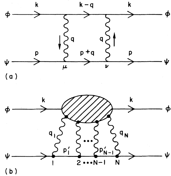
FIG. 1. (a) The box diagram that could give rise to an effective \phi^{\dagger}\phi\bar{\psi}\psi term; and (b) its higher-order iterations.
