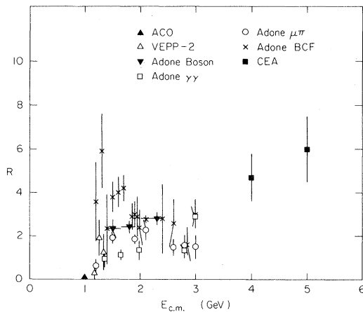
FIG. 1. Earlier measurements of the ratio R = \sigma_{\text{had}}/\sigma_{\mu\mu} as a function of the c.m. energy E_{c.m.} from Frascati (Adone) (Ref. 1), Orsay (ACO) (Ref. 2), Novosibirsk (VEPP-2) (Ref. 3), and Cambridge (CEA) (Ref. 4).
