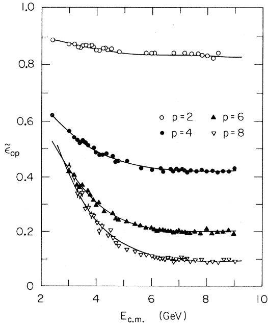
FIG. 6. Detection-efficiency matrix elements \tilde{\epsilon}_{0p} versus the c.m. energy E_{c.m.} , where \tilde{\epsilon}_{0p} is the probability that an event produced with p charged particles is not detected.
