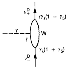
FIG. 5. A helicity-flipping transition involving the action of a right-handed current of strength r . The amplitude for this transition does not vanish when m \rightarrow 0 .
