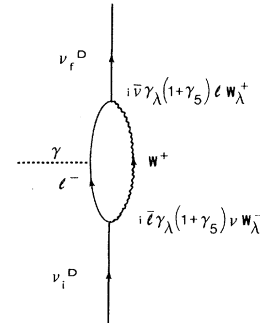
FIG. 2. One-loop diagram for the electromagnetic interaction of a Dirac neutrino \nu^D with initial momentum and spin projection values i and final ones f . The term in the weak Lagrangian which is active at each vertex is written next to it.
