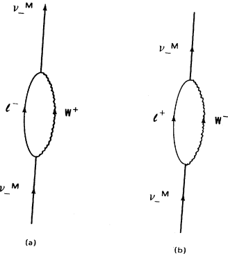
FIG. 1. Virtual components in the state of a Majorana neutrino \nu^M , whose subscript denotes its helicity. In the figure, l is a charged lepton and W the charged weak boson.
