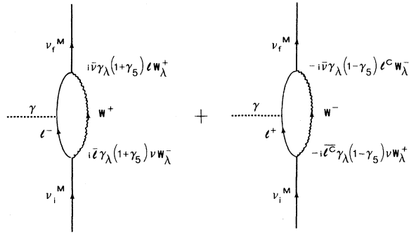
FIG. 3. One-loop diagrams for the electromagnetic interaction of a Majorana neutrino \nu^M . The symbol l^c denotes the charge conjugate of the field l .
