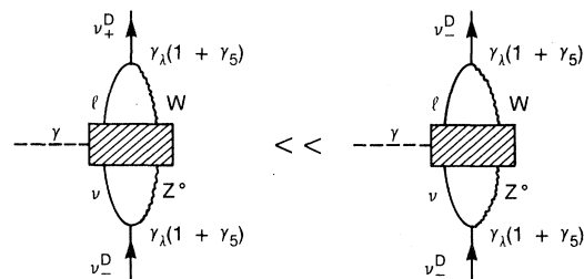
FIG. 4. Electromagnetic interactions of a highly relativistic Dirac neutrino, when all weak currents are left-handed, as indicated at the initial and final vertices. The symbol Z^0 denotes the neutral weak boson, and the shaded area an arbitrary structure.
