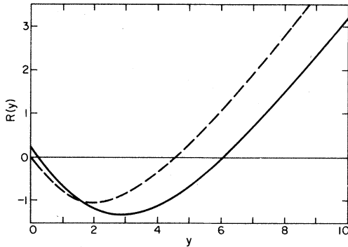
FIG. 4. The functions R(y) for the planar model in 2+1 dimensions. The continuous line is for four sites in a block, keeping three states at every site. The dashed line is for blocks of two sites and 21 states at every site.
