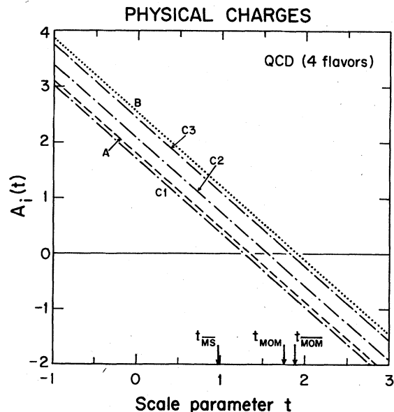
FIG. 1. Order- \alpha^2 coefficients A_i(t) for the physical charges \alpha_i^{\text{phys}} as a function of the scale-shift parameter t for QCD with four flavors of massless quarks.
