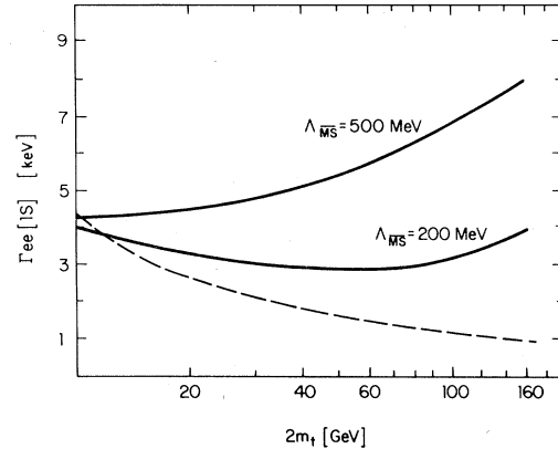
FIG. 7. Ground-state leptonic widths as a function of t -quark mass m_t . The solid lines correspond to the potentials of Fig. 5 and are based on Eq. (15) with a running coupling constant \alpha_s(2m_t) inferred from Fig. 3. The dashed line shows the results of Martin's potential (Ref. 12). Here we have ignored weak-interaction effects, which would only enhance the differences (cf. Figs. 13, 14, and Sec. VI).
