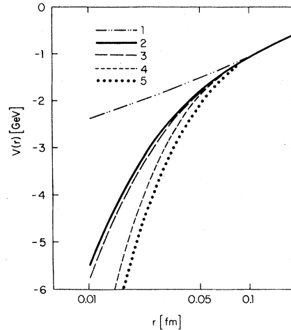
FIG. 2. The short-distance behavior of various potentials is shown. The numbers refer to the following references: (1) Martin, Ref. 12; (2) Buchmüller, Grunberg, and Tye, Ref. 13; (3) Richardson, Ref. 17; (4) Bhanot and Rudaz, Ref. 14; (5) Cornell group, Ref. 15.
