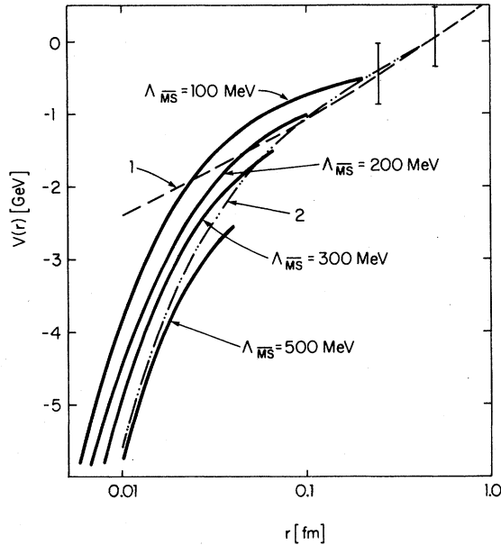
FIG. 4. Two-loop asymptotic-freedom potentials for four flavors and different values of \Lambda_{\overline{\text{MS}}} at distances r \leq r_c , r_c^2 = 1/(100\Lambda_{\overline{\text{MS}}}^2) . For comparison the potentials (1) and (2) of Fig. 2 are also displayed. The "error bars" indicate the uncertainty with respect to absolute normalization.
