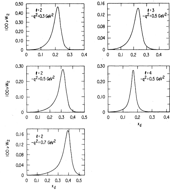
FIG. 3. Contribution of the resonances to the structure function \nu W_2 for different l and q^2 values, calculated using a (pion-nucleon-nucleon) three-body bound-state model.
