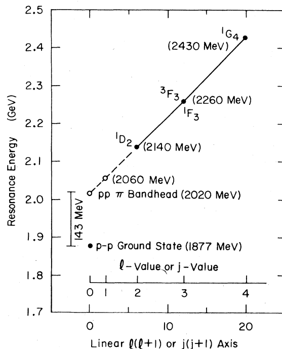
FIG. 1. Extrapolation used in Ref. 2 in order to find the l=0 and l=1 resonances.
