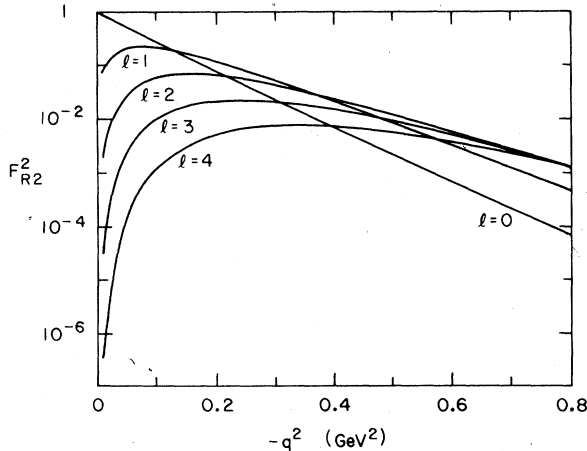
FIG. 2. Transition form factors (squared), calculated using a (nucleon-nucleon) two-body bound-state model for the resonances.
