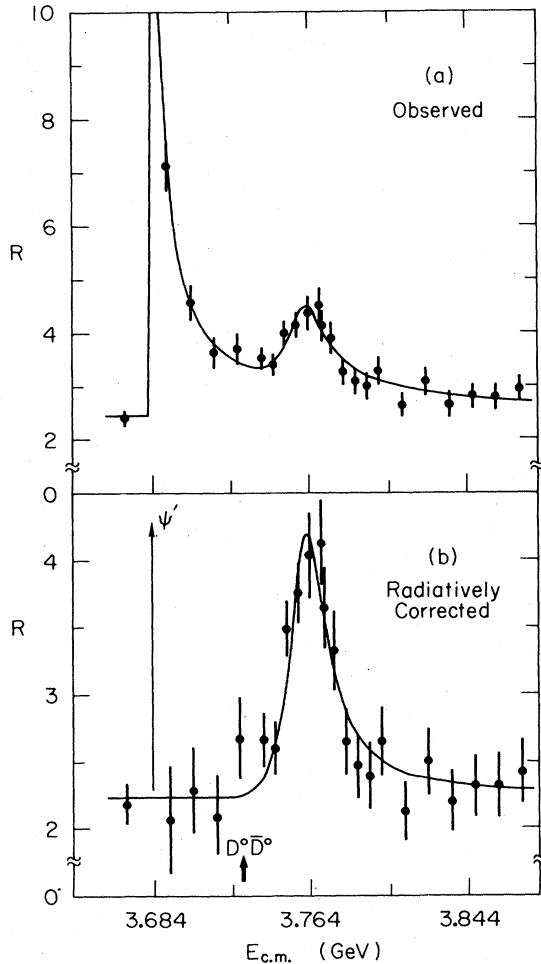
FIG. 1. (a) The observed cross section R (= \sigma_{hadronic} / \sigma_{\mu\mu}) with continuum radiative correction near the \psi(3770) . The curve is the fit to the data. (b) The cross section in units of R after radiative corrections for \psi(3095) , \psi(3684) , and \psi(3770) . The curve is the fitted Breit-Wigner form.
