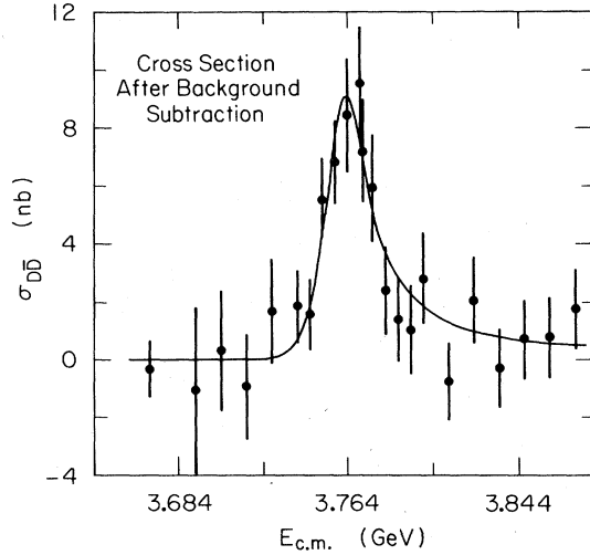
FIG. 2. The observed cross section for D\bar{D} production.
