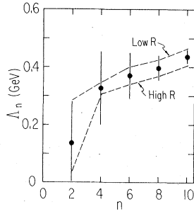
FIG. 31. Variation of \Lambda_n with n in second order QCD analysis. Low R means R=0.11 for ep , 0.17 for \mu p . High R means R=0.31 for ep , 0.87 for \mu p . Every point represents the same data set and carries its full statistical weight. The point-to-point errors are much smaller.
