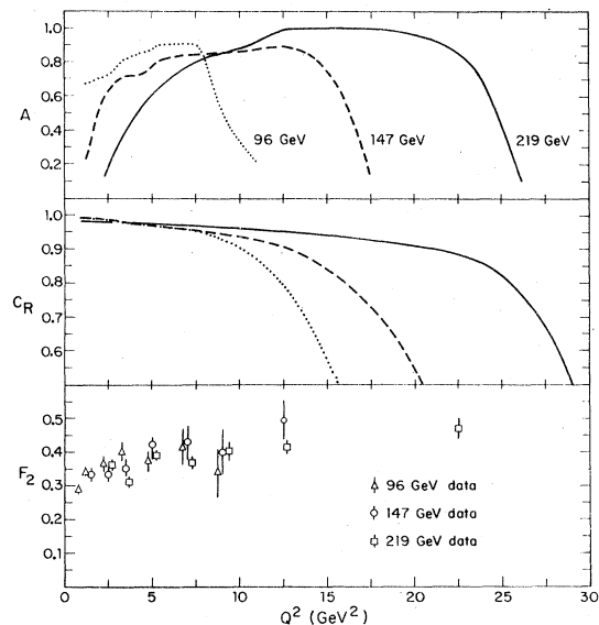
FIG. 14. Values of the acceptance, A , the inelastic radiative correction C_R , and the extracted structure function F_2 versus Q^2 for 9 < \omega < 20 .
