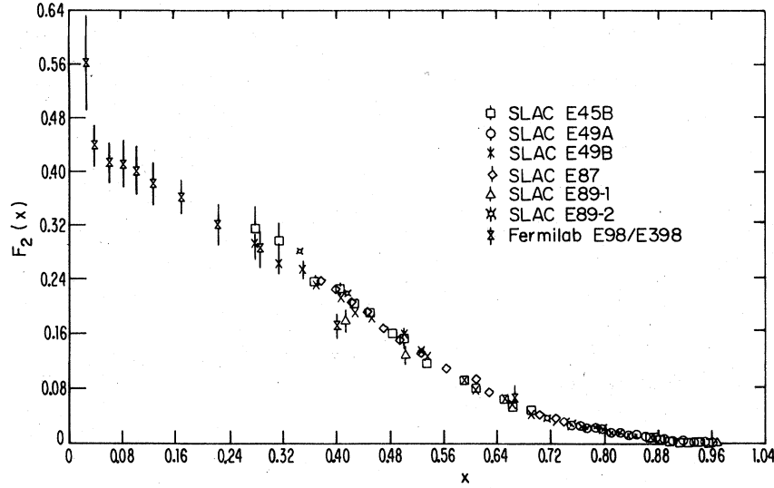
FIG. 25. Sample plot of data with 8 \leq Q^2 \leq 10 \text{ GeV}^2 used to obtain the moments of F_2 at Q^2 = 9 \text{ GeV}^2 . The \mu p data are from Fermilab E98/398. The ep data are from SLAC experiments as indicated. The value of R was taken to be 0.52 for \mu p , 0.21 for ep .
