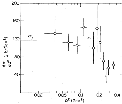
FIG. 22. d\sigma/dQ^2 = (\sigma_T + \epsilon_{ST}) as a function of Q^2 for 319 < W^2 < 375 \text{ GeV}^2 .
