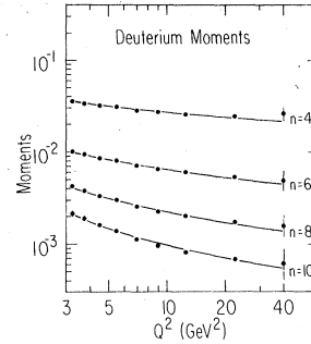
FIG. 29. The experimental Nachtmann moments for n=4 to n=10 for deuterium and the fit in leading-order QCD. Each n analyzed separately at Q_0^2=10 GeV 2 .
