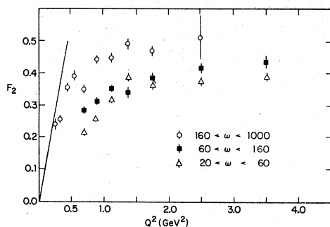
FIG. 20. F_2 for hydrogen as a function of Q^2 for several bands of \omega . The line is the constraint on the low- Q^2 variation of F_2 imposed by the real photon cross section.
