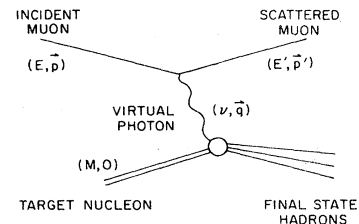
FIG. 1. Feynman diagram for one-photon exchange.
