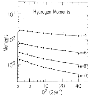
FIG. 28. The experimental Nachtmann moments for n=4 to n=10 for hydrogen and the fit in leading-order QCD. Each n analyzed separately at Q_0^2=10 GeV 2 .
