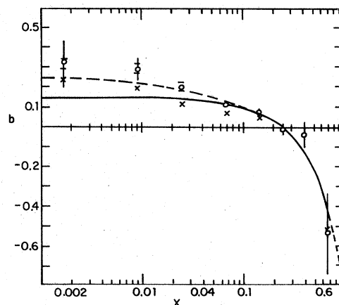
FIG. 21. The scaling-violation parameter b of Eq. (13) as a function of x for all muon-proton scattering data in this experiment. The horizontal bars indicate the change in b as R is changed from the central value of 0.52 to 0.69 or 0.37. The crosses are the values that would be obtained if we set R=0 . The errors are statistical only. The line is part of a global fit to the data using b(x) = c_1 + c_2 \ln(1-x) [Eq. (14)]. Also shown (dashed) is the simpler form b(x) = 0.25 - x (Ref. 17).
