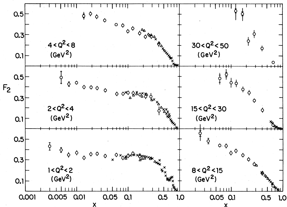
FIG. 19. F_2 for hydrogen as a function of x for various Q^2 bins, using R=0.52 . Additional SLAC and MIT-SLAC points have been added.
