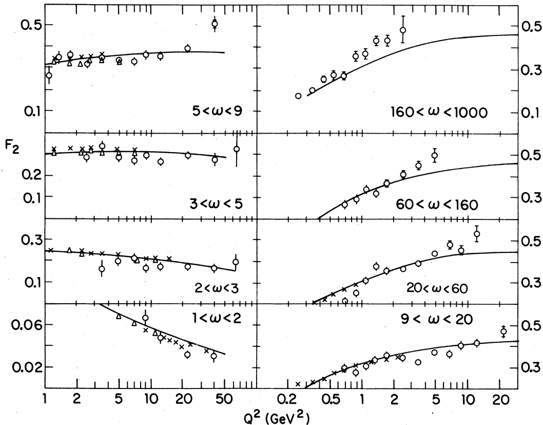
FIG. 24. F_2 for hydrogen as a function of Q^2 , showing the data of Fig. 18. The lines are the results of fits to the approach-to-scaling and scaling regions of Eq. (15).
