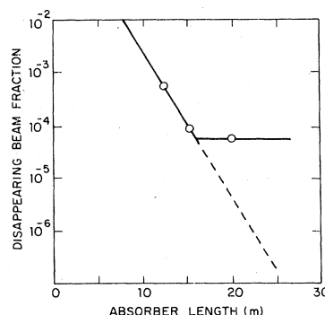
FIG. 3. Fraction of beam absorbed in steel hadron absorber as a function of polyethylene absorber length in D3 magnets.
