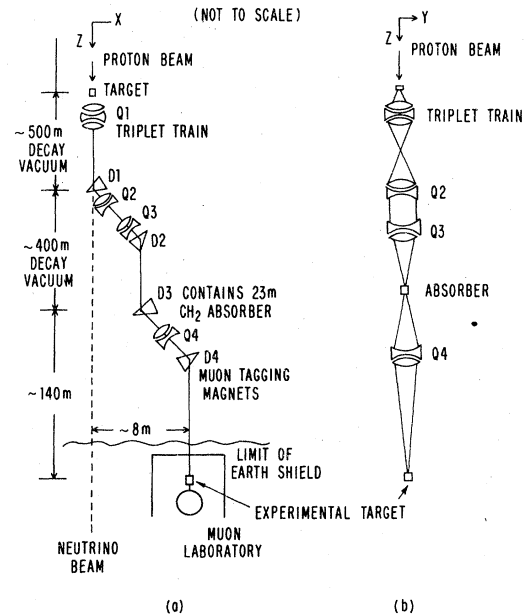
FIG. 2. Schematic diagram of Fermilab muon beam and beam optics.
