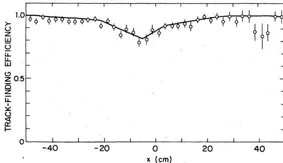
FIG. 12. Track-finding efficiency across the 6-m chambers for the 219-GeV data.
