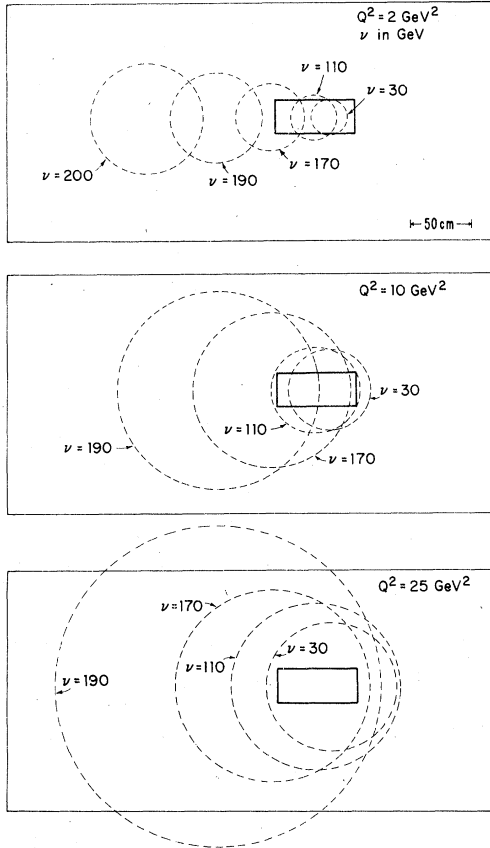
FIG. 11. Position of muons with constant Q^2 , for several values of \nu at the muon hodoscopes for the 219-GeV data. Positive x is to the right in these diagrams.
