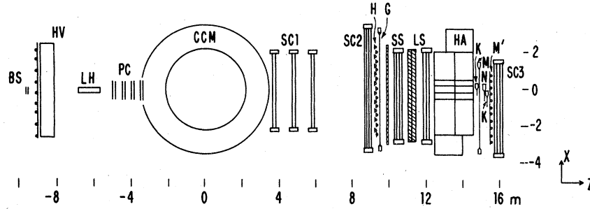
FIG. 6. Experimental apparatus seen from above. The muon beam enters at left. BS: last beam station; HV: halo veto wall and hodoscope; LH: liquid hydrogen target; PC: multiwire proportional chambers; CCM: Chicago cyclotron magnet; SC1: Shift-register chambers; SC2: 6-m chambers; H: H hodoscope; G: G hodoscope; SS: Steel wall and spark chambers for photon and electron detection; LS: lead wall and spark chambers for hadron identification; HA: steel hadron absorber; K: beam veto hodoscope; M, N, M' : muon hodoscopes; SC3: muon spark chambers.
