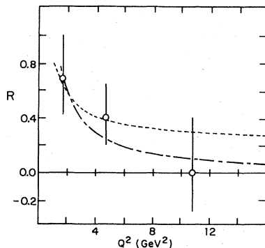
FIG. 17. Extracted values of R vs Q^2 . The dashed curve is R = 1.18(1-x)/\ln(Q^2/\Lambda^2) with \Lambda = 0.5 \text{ GeV} ; the other curve is R = 1.20(1-x)/Q^2 .
