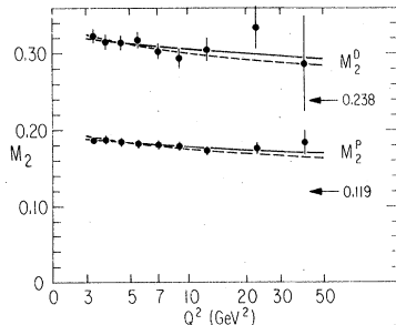
FIG. 26. Energy-momentum sum rule. The experimental Nachtmann moments M_2(Q^2) for hydrogen and deuterium. Leading-order QCD fits are shown. Solid curve is for \Lambda=0.24 GeV, dashed curve for \Lambda=0.61 GeV. The values 0.238 and 0.119 indicated by the arrows are the asymptotic Q^2 \rightarrow \infty limits expected for the four-flavor, three-color quark-gluon model in QCD.
