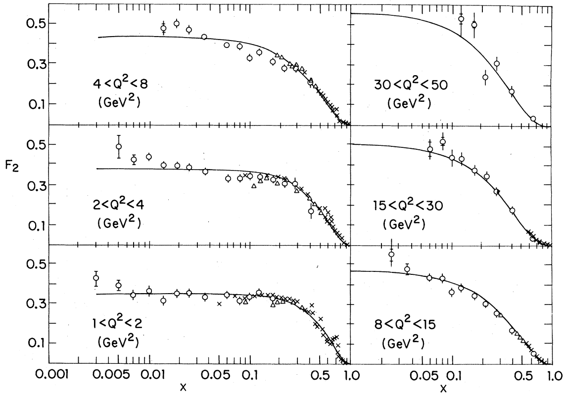
FIG. 23. F_2 for hydrogen as a function of x , showing the data of Fig. 19. The lines are the results of the global fit to the scaling region of Eq. (14).
