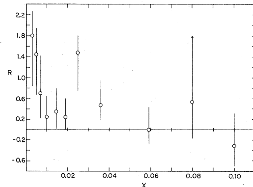
FIG. 16. Extracted values of R vs x using the data-comparison technique. The average value of Q^2 for each point is different, and decreases with x .
