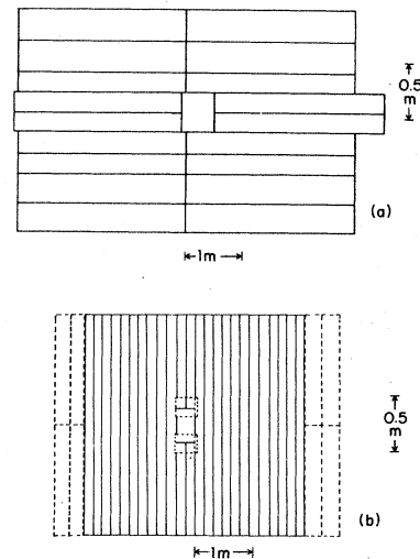
FIG. 7. Dimensions of (a) G and (b) H hodoscopes.
