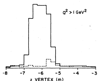
FIG. 9. Vertex distribution of analyzed events. Solid line: full target. Dotted line: empty target normalized to the same incident muon flux.
