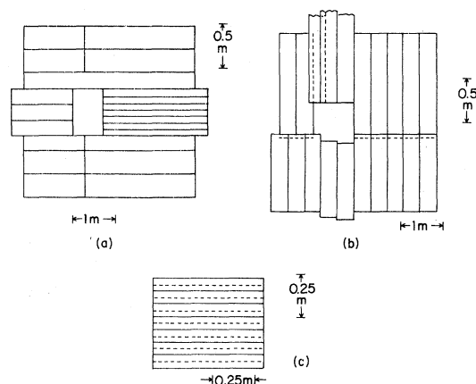
FIG. 8. Dimensions of (a) M , (b) M' , and (c) N hodoscopes. In the figure dotted lines show edges behind other counters.
