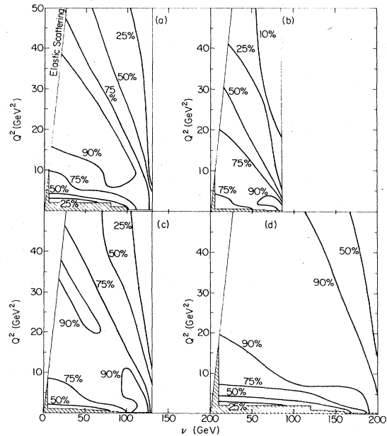
FIG. 10. Contours of constant acceptance for (a) runs 1 and 3, 147-GeV data; (b) run 2, 96-GeV data; (c) run 4, 147-GeV data; (d) run 5, 219-GeV data.
