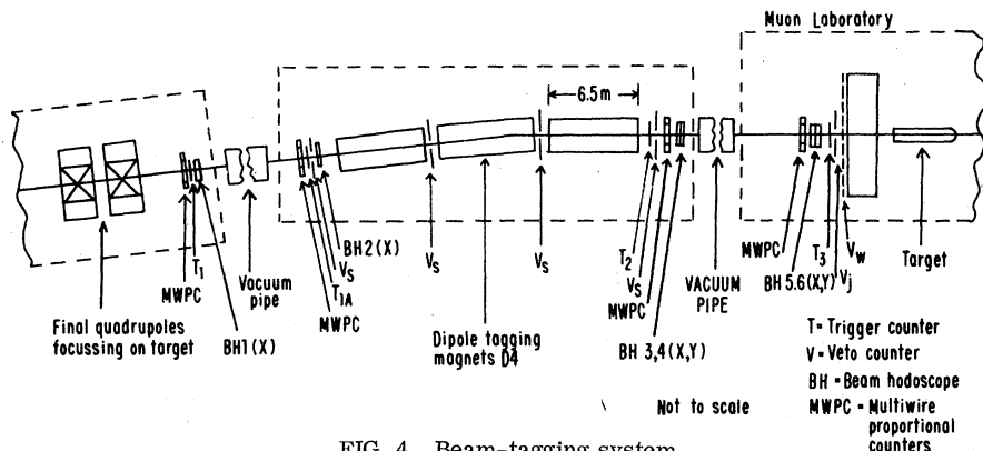
FIG. 4. Beam-tagging system.
