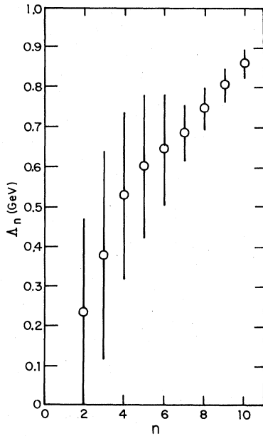
FIG. 27. Variation of \Lambda_n with n in leading-order QCD analysis. Every point represents the same data set and carries its full statistical weight. The point-to-point errors are much smaller.
