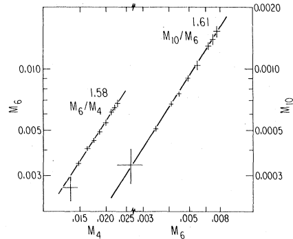
FIG. 30. Plot of \log M_6(Q^2) versus \log M_4(Q^2) and \log M_{10}(Q^2) versus \log M_6(Q^2) .
