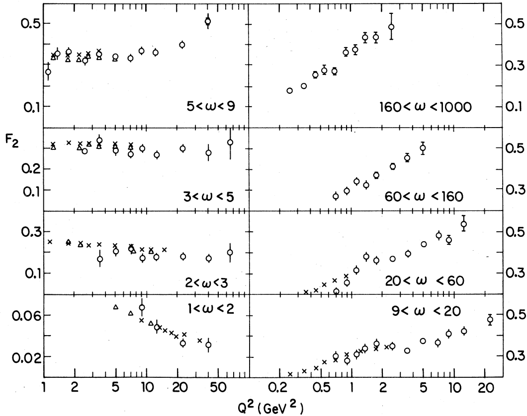
FIG. 18. F_2 for hydrogen as a function of Q^2 for various \omega bins, using R = 0.52 , showing the combined Fermilab data (circles), the MIT-SLAC data (triangles) (Ref. 28), and the SLAC data (crosses) (Ref. 33). The errors shown are statistical only. The horizontal bars indicate the effects of changing R to 0.69 and 0.37. Note the differences in scale and suppressed zeros on the ordinates.
