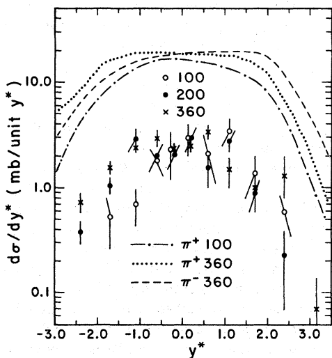
FIG. 8. The c.m. rapidity distributions d\sigma/dy^* for \rho^0 mesons at 100 ( \circ ), 200 ( \bullet ), and 360 ( \times ) GeV/c. Also shown for comparison are d\sigma/dy^*(\times 0.1) for \pi^+p \rightarrow \pi^+X^- at 100 and 360 GeV/c and for \pi^-p \rightarrow \pi^-X^+ at 360 GeV/c.
