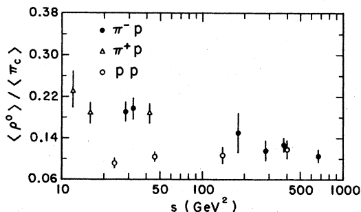
FIG. 6. The ratio \langle \rho^0 \rangle / \langle \pi_c \rangle (see text) as a function of s for \pi^+p and pp interactions.
