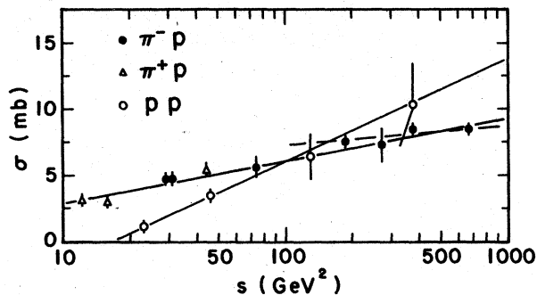
FIG. 3. Inclusive \rho^0 production cross sections as a function of s for \pi^\pm p interactions. The solid lines represent the fits to all the data described in the text. The dashed line represents the fit to the \pi^-p data above s = 100 \text{ GeV}^2 .
