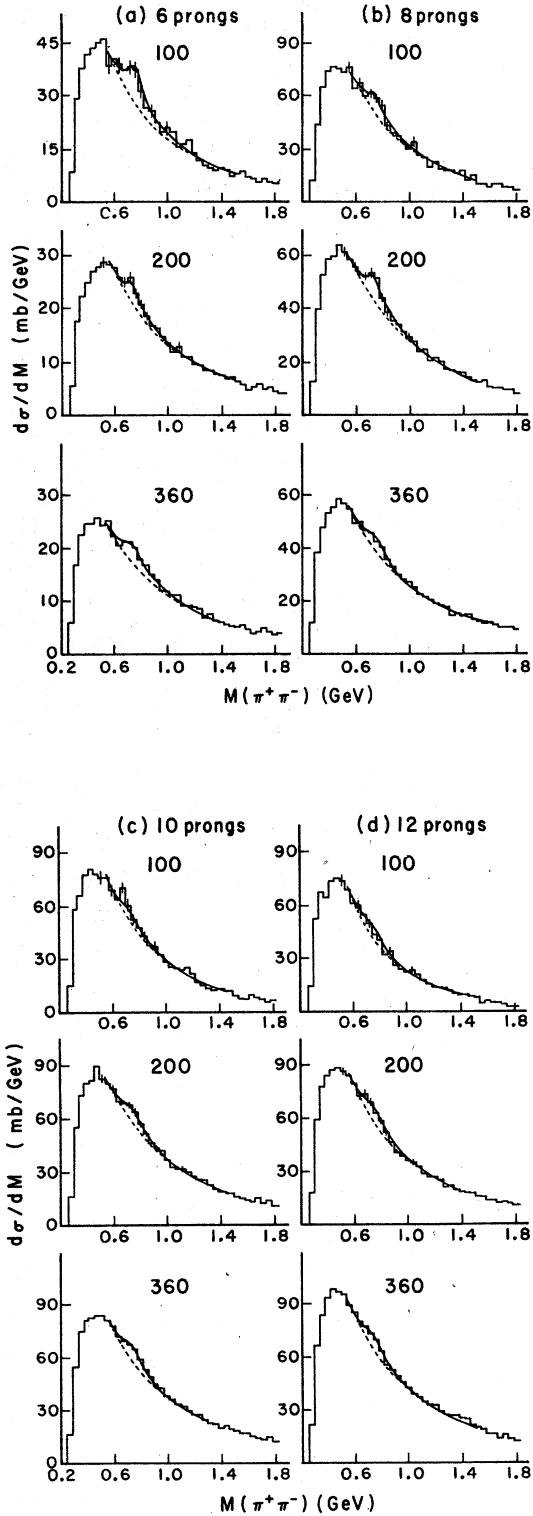
FIG. 2. Semi-inclusive \pi^+\pi^- mass distributions for (a) n=6 , (b) n=8 , (c) n=10 , and (d) n=12 in 100-, 200-, and 360-GeV/c \pi^+p interactions. The solid curves represent fits described in the text. The dashed curves indicate the background contributions.
