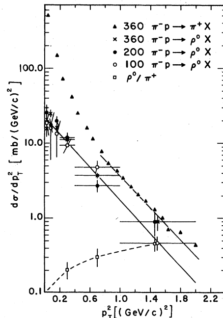
FIG. 7. Distributions of d\sigma/dp_T^2 for \rho^0 mesons in 100-, 200-, and 360-GeV/c \pi^-p interactions and for \pi^+ mesons in 360-GeV/c \pi^-p interactions. The lines represent fits described in the text.
