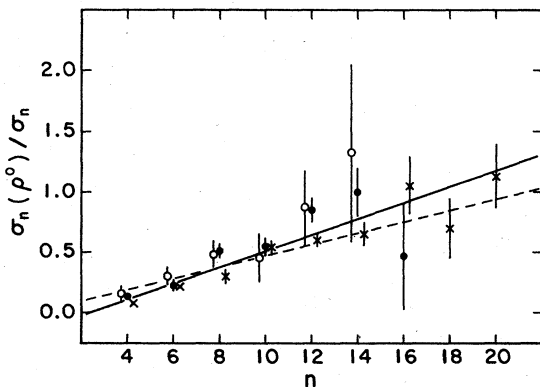
FIG. 5. Values of \langle \rho^0 \rangle_n = \sigma_n(\rho^0)/\sigma_n as a function of charge multiplicity n for 100 (○), 200 (●), and 360 (×) GeV/c \pi^-p interactions. The lines represent fits described in the text.
