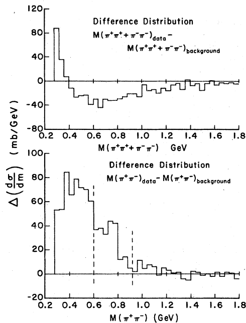
FIG. 9. Distributions of the difference between experimental distributions of M(\pi\pi) and background distributions of pion pairs constructed from pions selected from different events of the same charge multiplicity in 360-GeV/c \pi^-\bar{p} interactions. The background distributions are normalized to the data in the mass region 2.0 < M(\pi\pi) < 4.0 GeV. Difference distributions are shown for pion pairs of like and unlike charge.
