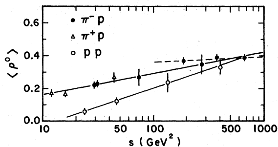
FIG. 4. The average number of \rho^0 mesons per inelastic event \langle \rho^0 \rangle , plotted as a function of s for \pi^\pm p and pp interactions. The solid lines represent the fits to all the data described in the text. The dashed line represents the fit to the \pi^-p data above s = 100 \text{ GeV}^2 .
