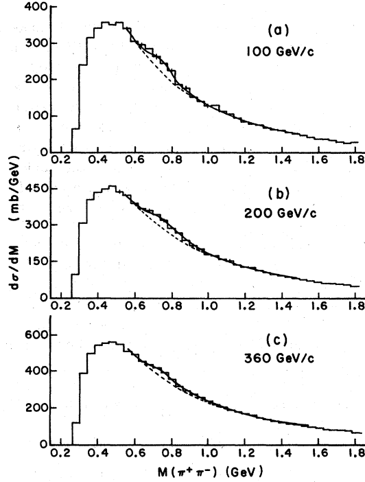
FIG. 1. Inclusive \pi^+\pi^- mass distributions for the process \pi^-p \rightarrow (\pi^+\pi^-)X^0 at (a) 100, (b) 200, and (c) 360 GeV/c. The solid curves represent fits to the data as described in the text. The dashed curves indicate the background contributions.
