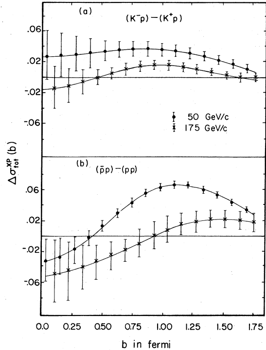
FIG. 31. \Delta\sigma_{\text{tot}}^{xp}(b) for (a) Kp and (b) \bar{p}p at p = 50 GeV/c (circles) and at p = 175 GeV/c (crosses).
