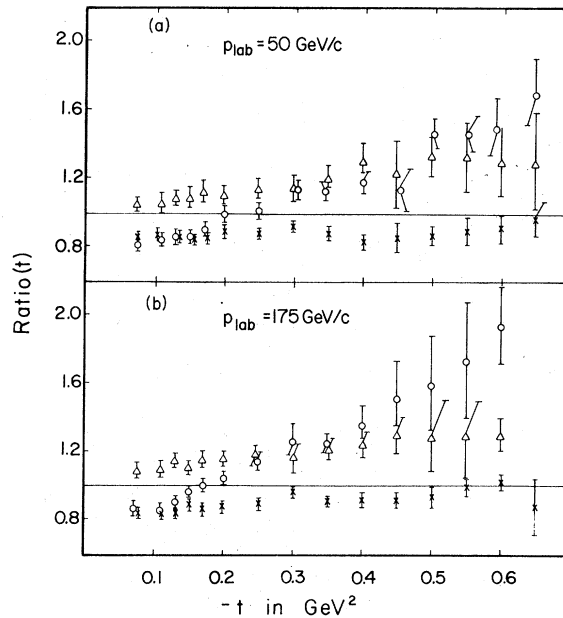
FIG. 32. Quark-model ratios at (a) p = 50 GeV/c and (b) p = 175 GeV/c. The different ratios are (circles) \frac{2}{3}S(Kp)/S(p p) (crosses) S(Kp)/S(\pi p) , and (triangles) S(\pi p)/[\frac{1}{2}S(Kp) + \frac{1}{3}S(p p)] .
