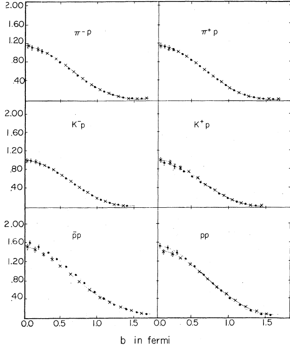
FIG. 27. \text{Im}h_{\text{el}}(s, b) for the six reactions at 50 GeV/c (circles) and at 175 GeV/c (crosses). The errors shown include the statistical errors, the uncertainty due to the real part and to large- t contributions ( 0.75 \leq |t| \leq 1.4 GeV 2 ).
