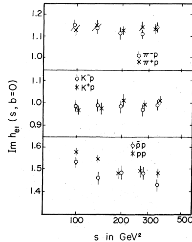
FIG. 28. \text{Im}h_{\text{el}}(s, b=0) as a function of s for \pi^\pm p , K^\pm p , and p^\pm p . The errors are calculated as for Fig. 27.
