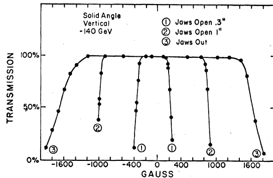
FIG. 7. Curves of the 0^\circ spectrometer transmission through the aperture-defining jaw counters for three settings of the jaws as a function of the incident beam angle measured in field strength of the scattering angle magnet system. The ratio of the FWHM for curves 1 and 2, 0.306, compared with the ratio of the jaw openings, 0.305, is a check on the measurement. Curve 3 shows the physical aperture of the spectrometer as defined by magnet steel when the jaws are fully open.
