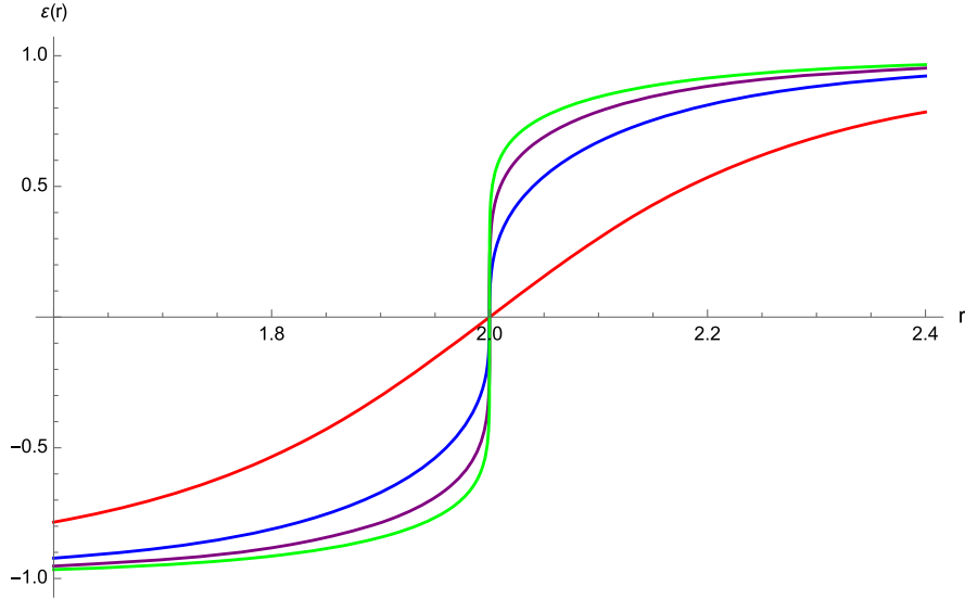
FIG. 2. The approximating function (23) with M = 1 , \rho = 0.1M^2 , and \kappa = 0 (red curve), \kappa = 1 (blue curve), \kappa = 2 (purple curve), and \kappa = 3 (green curve). The plot shows that larger values of \kappa result in a steeper function around r = 2M .
