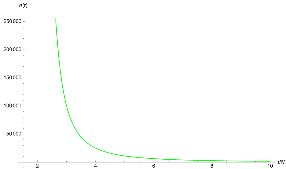
FIG. 5. Proper time \sigma(r) of a radially accelerated observer obtained by numerically solving the differential equation (62) with the initial condition \sigma(r_0) = 0 . The functions \varepsilon and \mathcal{F} have been evaluated by employing Eqs. (23) and (64), respectively. The solution \sigma(r) diverges at the event horizon.
