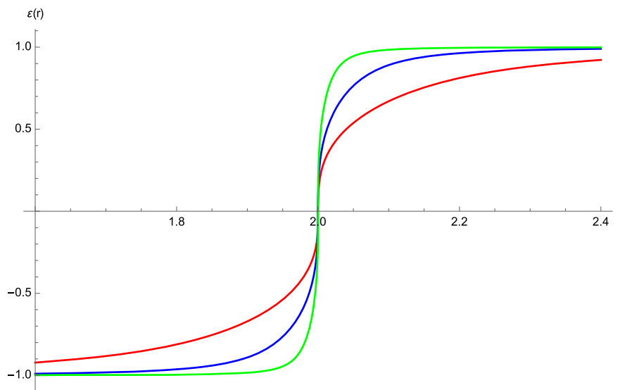
FIG. 1. The approximating function (23) with M = 1 , \kappa = 1 , and \rho = 0.1M^2 (red curve), \rho = 0.01M^2 (blue curve), and \rho = 0.001M^2 (green curve). It is clear that \epsilon(r) gets sharper in the neighborhood of r = 2M as \rho approaches zero.
