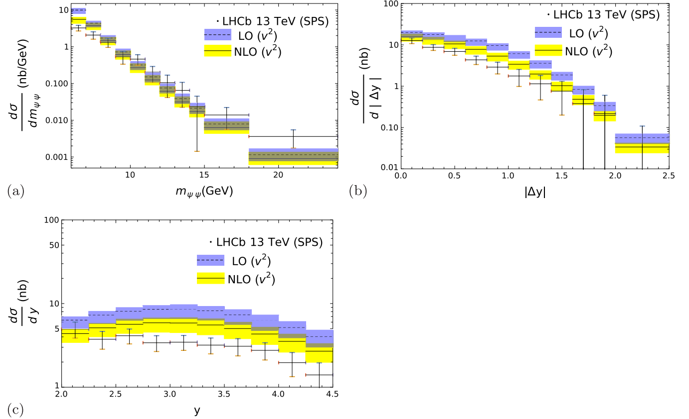
FIG. 1. The (a) m_{\psi\psi} , (b) |\Delta y| , and (c) y distributions of prompt double J/\psi hadroproduction in SPS measured by LHCb [15] at \sqrt{s} = 13 \text{ TeV} are compared with our CS NRQCD predictions at LO (dashed lines) and NLO with respect to relativistic corrections (solid lines). The theoretical uncertainties are indicated by the shaded blue (LO) and yellow (NLO) bands.
