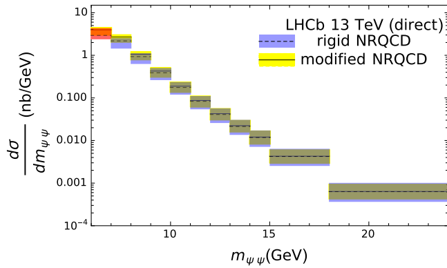
FIG. 2. The m_{\psi\psi} distribution of direct double J/\psi hadroproduction in SPS under LHCb experimental conditions adopting NRQCD with \mathcal{O}(v^2) relativistic corrections evaluated in our modified approach (solid lines) is compared with its counterpart obtained by rigidly expanding the phase space in v^2 (dashed lines). The theoretical uncertainties are indicated by the shaded blue (rigi-NRQCD) and yellow (our NRQCD) bands. Negative values are shown in red.
