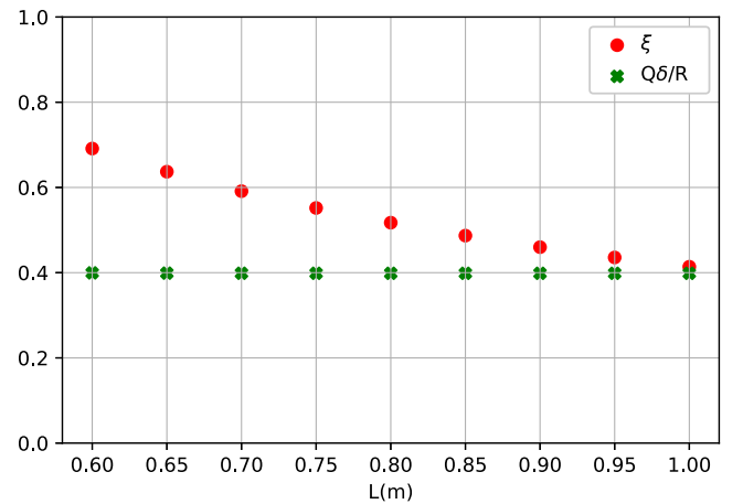
FIG. 8. Dependence of \xi and Q\delta/R on the length of the cavity L . Note that the product of \xi and L and Q\delta/R are very nearly constant, consistent with the statement that the part of the cavity away from the post can be removed without affecting the mode of interest.
