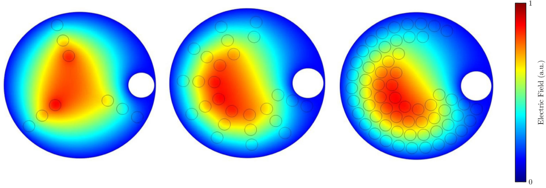
FIG. 21. Simulation of a cavity of radius 0.325 m loaded with different numbers of sapphire dielectric rods, each 12.5 mm in radius, and a metallic tuning rod. Dielectric loading enables the cavity to cover the frequency range 165–370 MHz. (a) 286.43 MHz resonant mode with 9 rods, (b) 216.73 MHz resonant mode with 26 rods, and (c) 164.59 MHz resonant mode with 61 rods.
