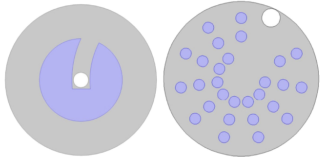
FIG. 20. Cross sectional view of dielectric loaded cavities. (a) Cavity loaded with a large ceramic cylinder machined to allow movement of a metallic tuning rod. The rod is at the cavity center. (b) Cavity loaded with 28 ceramic rods arranged to allow movement of a metallic tuning rod. The rod is at the cavity wall.
