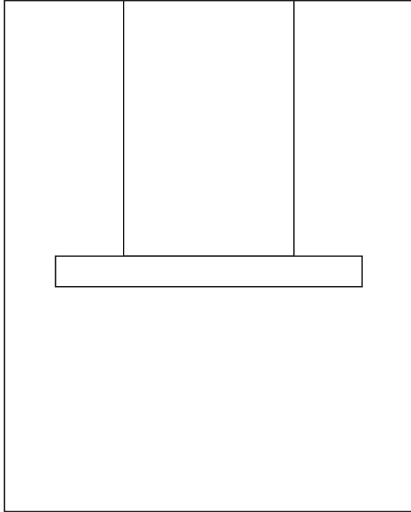
FIG. 9. Reentrant cavity with movable post and disk.
