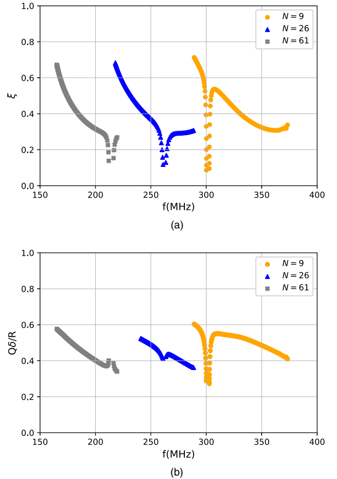
FIG. 22. (a) \xi and (b) Q\delta/R versus frequency for the different dielectric loading configurations described in Fig. 20. The dip in each curve is due to mode crossing, and mixing, with a TE mode.
