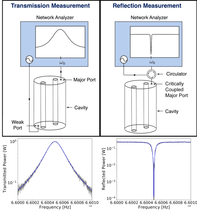
FIG. 5. Sample transfer functions of the resonant cavity around well-coupled mode (TM 010 -like). The mode is centered at 660.05 MHz. Left-top: illustration of the mode transmission function S_{12} from the weak port through the main port with a Lorentzian envelope about the mode center [Eq. (4)]. Bottom: example S_{12} scan with fit Lorentzian with the cavity at sub-Kelvin temperature. Right-top: illustration of the mode reflection function S_{11} in/out of the main port with envelope of the form in Eq. (8). Bottom: example S_{11} scan with the best fit envelope with cavity at sub-Kelvin temperature.
