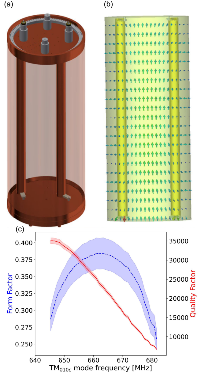
FIG. 4. ADMX main cavity and TM_{010} -like simulated mode properties: (a) view of the interior of the main cavity; (b) TM_{010} -like mode electric field in side view; (c) simulated mode form factor (blue dashed) and measured cyogenic loaded quality factor (red solid) over the Run 1A tuning path. Errors (shaded regions) in the form factor and quality factor were computed to be 6% and 2.2% respectively, as discussed in Sec. IV E and presented in Table I.
