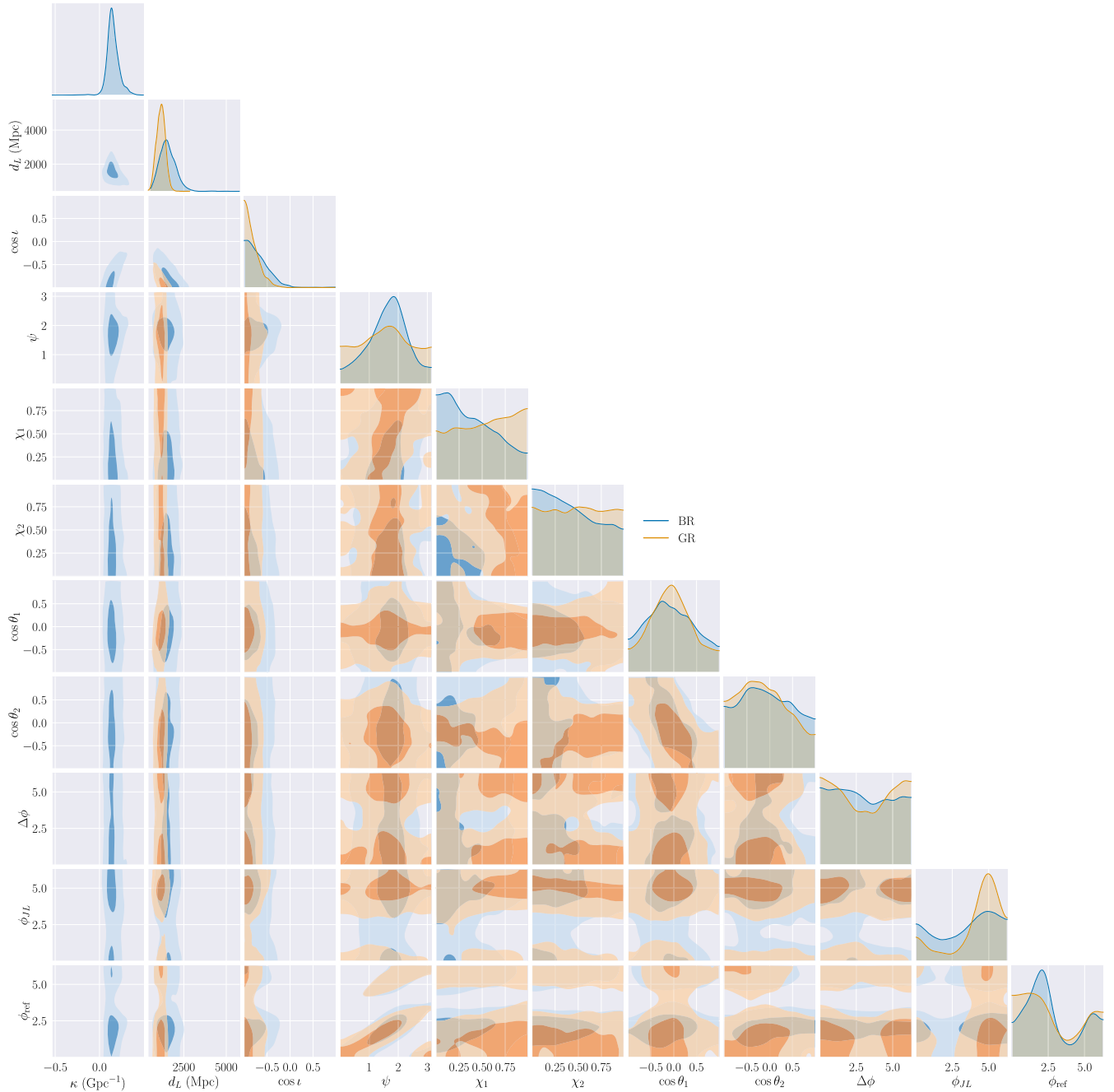
FIG. 11. Extended corner plot for GW170818: a supplement to Fig. 6 discussed in Appendix A 1. The shaded regions contain 90% and 39.35% ( 1\sigma ) of the probability mass. The prior is uniform in all shown quantities except d_L , whose prior corresponds to a distribution uniform in comoving volume.
