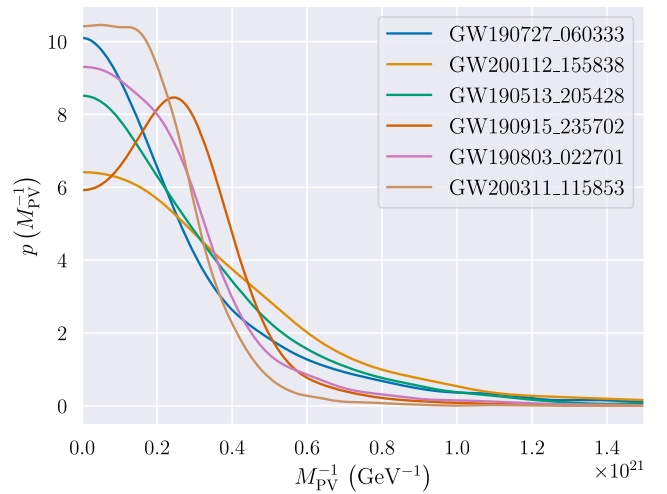
FIG. 9. Individual-event M_{\text{PV}}^{-1} posteriors from our analysis, converted from the \kappa posteriors in Fig. 2 via Eq. (16). Chosen events are those highlighted in Fig. 1 of Zhu et al. [19].
