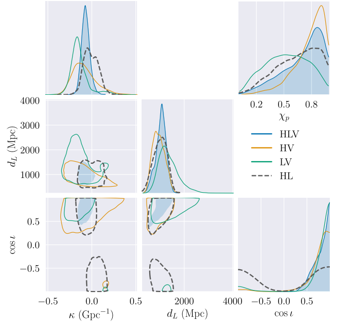
FIG. 8. GW200129 posterior on \kappa , luminosity distance d_L , and inclination \cos \iota , including different sets of detectors in the analysis per the legend. The marginalized posterior on \chi_p is shown in the top right panel. The main run with all three detectors (HLV, filled blue), shows a preference for \kappa < 0 , as in Fig. 2; this preference is more pronounced for two-detector runs that include Virgo (HV and LV, orange and green); however, it disappears if we remove Virgo (HL, dashed black). The 2D contours correspond to the 90% credible level.
