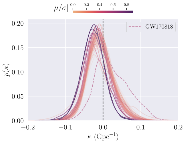
FIG. 4. Individual-event \kappa_i distributions of Fig. 2 reweighted in light of the population-level inference of Fig. 3, marginalizing over \mu and \sigma . Curves are colored by the magnitude of the supported deviation, as represented by the respective posterior |\mu_i/\sigma_i| .
