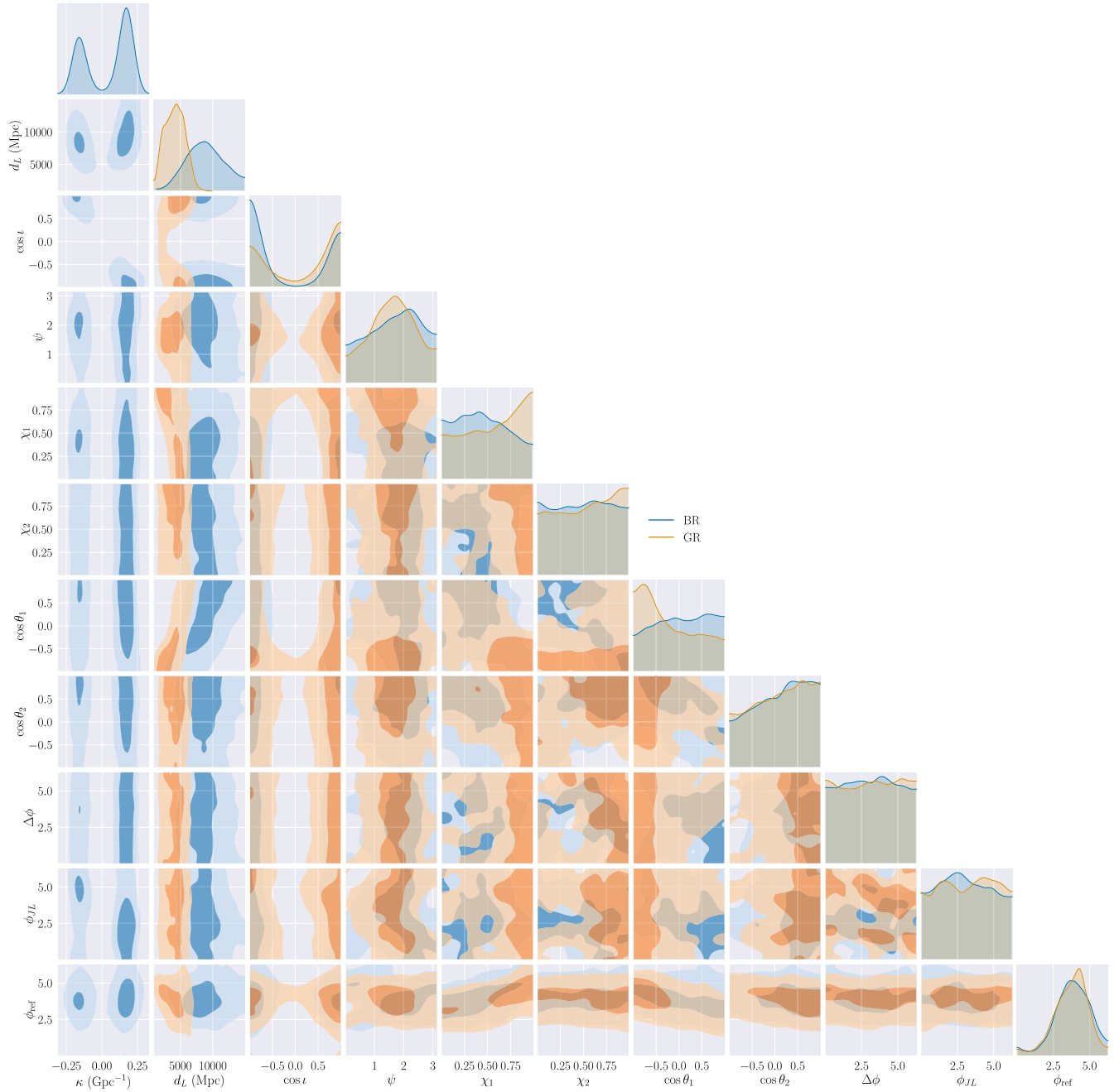
FIG. 12. Extended corner plot for GW190521: a supplement to Fig. 7 discussed in Appendix A 2. The shaded regions contain 90% and 39.35% ( 1\sigma ) of the probability mass. The prior is uniform in all shown quantities except d_L , whose prior corresponds to a distribution uniform in comoving volume.
