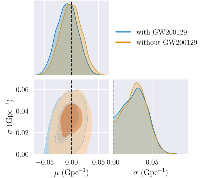
FIG. 3. The posterior of the \kappa population hyperparameters \mu and \sigma , including (blue) and excluding (orange) GW200129 from the collection of events. The two-dimensional (2D) contours correspond to the 39.35% and 90% credible levels. The plot shows that the population constraint on \kappa is consistent with no birefringence ( \mu = \sigma = 0 ) at the 90% credible level.
