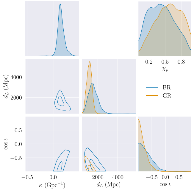
FIG. 6. GW170818 posterior on \kappa , luminosity distance d_L , and inclination \cos \iota from our birefringence analysis (blue), compared to the GR result (orange). The top right panel shows the marginalized posterior on \chi_p : allowing for birefringence reduces the preference for precession. (See Fig. 11 for a full corner plot).
