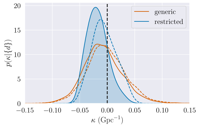
FIG. 5. Restricted and generic posteriors on \kappa , which, respectively, do and do not assume that \kappa is shared by all events (color). Solid (dashed) traces indicate the analysis included (excluded) GW200129. The black dashed line marks the absence of birefringence ( \kappa = 0 ). The shaded distribution is the primary result in this work (blue band in Fig. 2).
