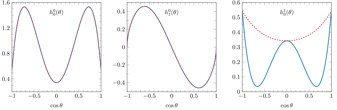
FIG. 2. Solid blue lines , moments obtained from the original waves of Table I; dotted red lines , moments obtained from the ambiguous solution of Table I. The polarized moment h_0^1 breaks the ambiguity between the two solutions.
