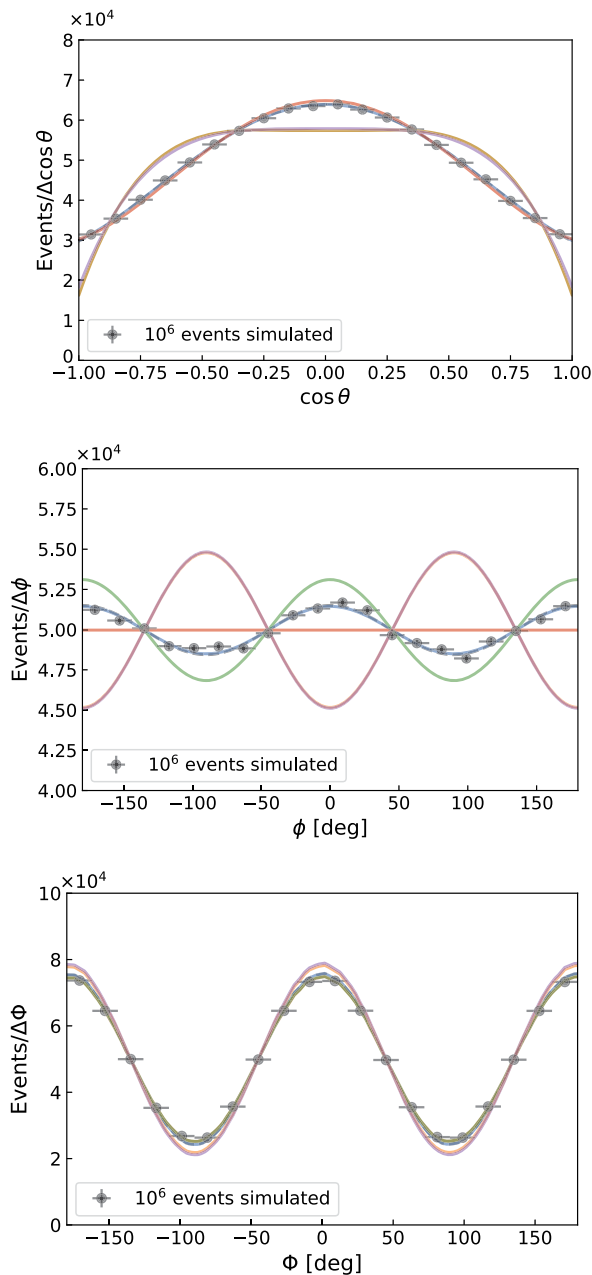
FIG. 8. As Fig. 4 for fits to 10^6 events with colors matching the plots in Fig. 7.
