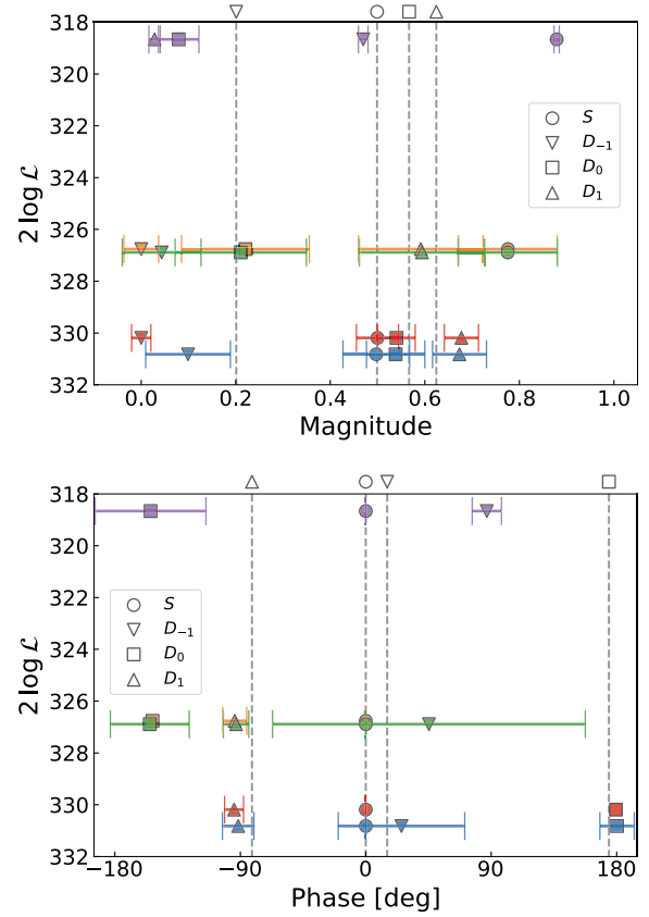
FIG. 3. Results of the 5 best (highest likelihood) fits from 50, to 100 events generated with the partial waves given in Table II showing the likelihood versus the amplitude magnitude (upper) and phase (lower), the dashed lines show the true values. The wave is indicated by the marker shape (see legend) while the color represents different solutions. The highest likelihood is at the bottom of the plots. The phase for the D_{-1} ( D_1 ) wave is not shown for the red and orange (purple) fits, as associated magnitude is zero and, hence, the phase is undetermined. Fits and uncertainties are computed using the HESSE option of MINUIT [19].
