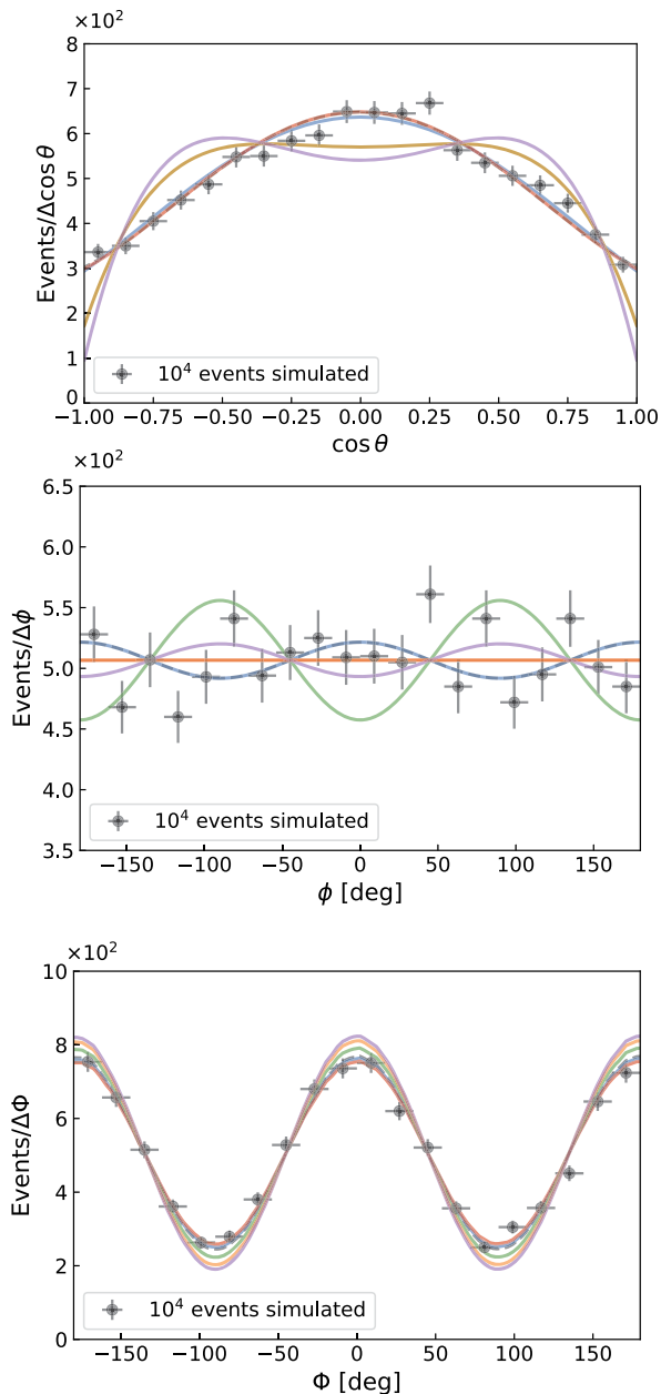
FIG. 6. As Fig. 4 for fits to 10^4 events with colors matching the plots in Fig. 5.
