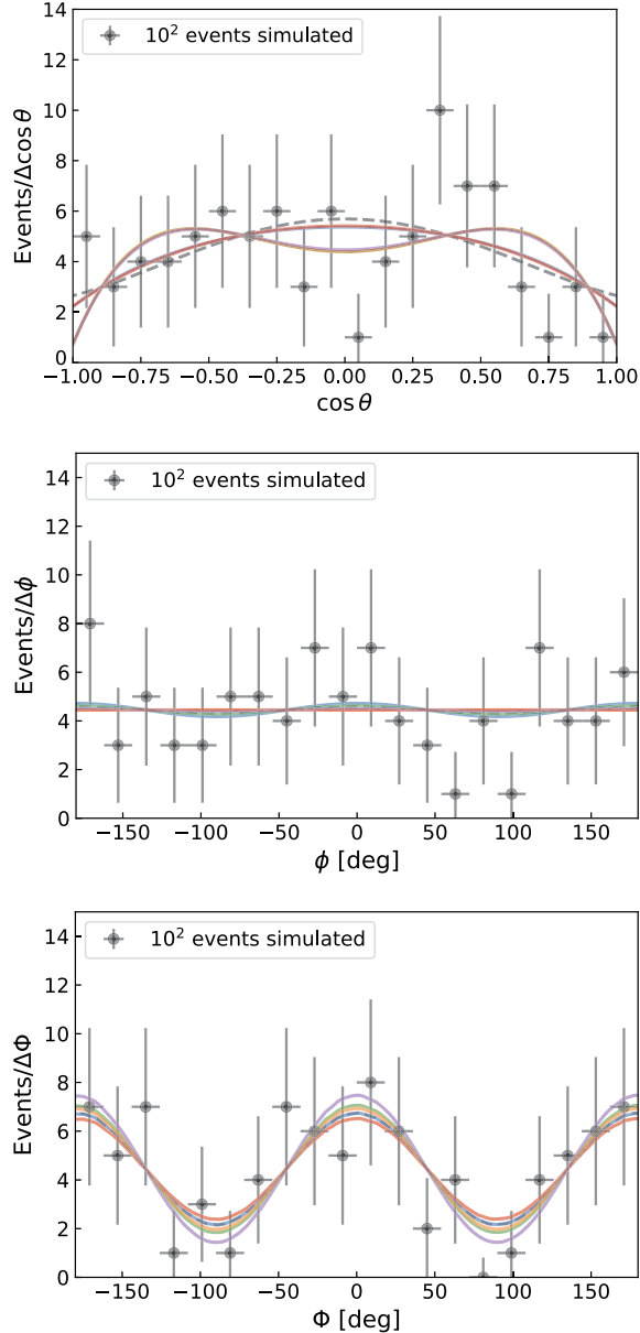
FIG. 4. Projections of the angular distributions (upper: \cos\theta , center: \phi , lower: \Phi ) as defined in Eqs. (5) and (8). Shown are the data (black circles), the true solution (dashed black), and the different solutions (colored lines), with colors matching the plots in Fig. 3. Bin widths are \Delta\cos\theta = 0.1 and \Delta\phi = \Delta\Phi = 18^\circ .
