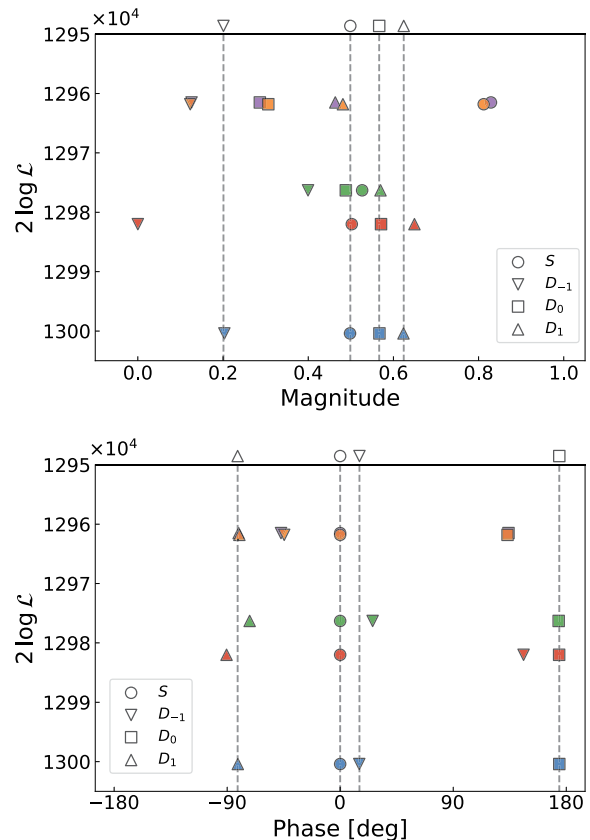
FIG. 7. As Fig. 3 for fits to 10^6 events. Uncertainties are negligible and not shown.
