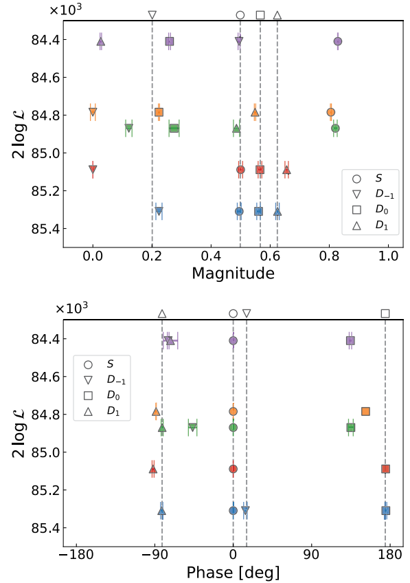
FIG. 5. As Fig. 3 for fits to 10^4 events. The phase for the D_{-1} wave is not shown for the red and orange fits, as associated magnitude is zero and, hence, the phase is undetermined.
