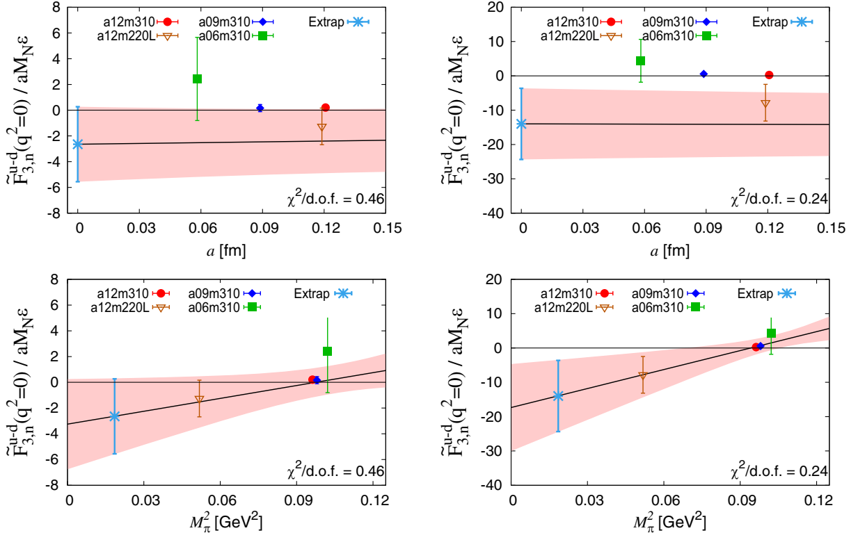
FIG. 10. Extrapolation to the continuum and physical pion mass limit using the fit ansatz c_1 + c_2M_\pi^2 + c_3a . Results from different ensembles are renormalized in \overline{\text{MS}} scheme at \mu = 2 GeV using Eq. (32). Left column shows the results from the “standard” excited-state fit, and the right column shows the results from the “ N\pi ” excited-state fits. Extrapolated values are \tilde{F}_3(0)/aM_N\epsilon = -2.6(2.9) for the “standard” excited-state fit, and \tilde{F}_3(0)/aM_N\epsilon = -14(10) for the “ N\pi ” excited-state fit.
