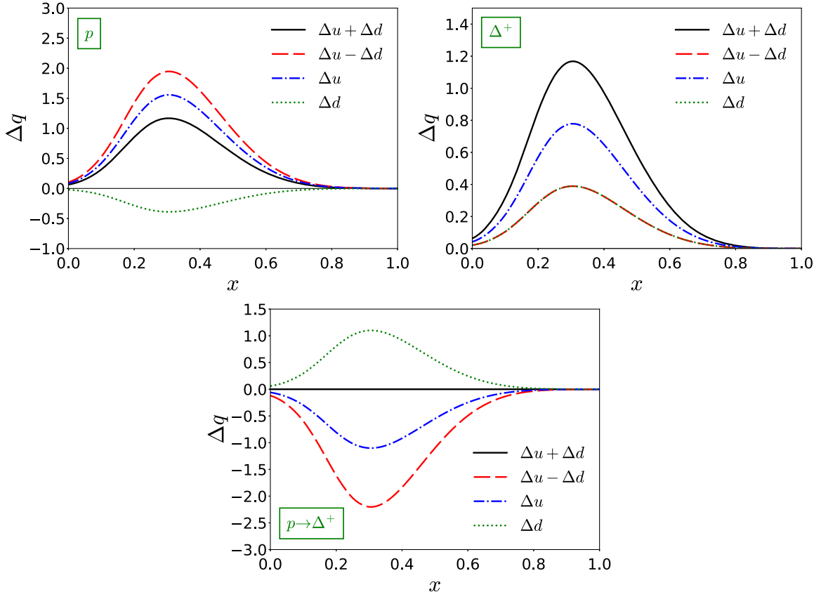
FIG. 1. Longitudinally polarized quark distribution functions for the proton (upper left panel), \Delta baryon (upper right panel), and p \rightarrow \Delta^+ transition (lower panel). The solid (black), dashed (red), dot-dashed (blue), and dotted (green) lines represent the \Delta u + \Delta d , \Delta u - \Delta d , \Delta u , and \Delta d contributions, respectively.
