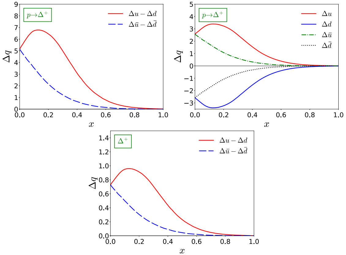
FIG. 3. Longitudinally polarized quark distribution functions for the p \rightarrow \Delta^+ (upper panels) and \Delta^+ baryon (lower panel).
