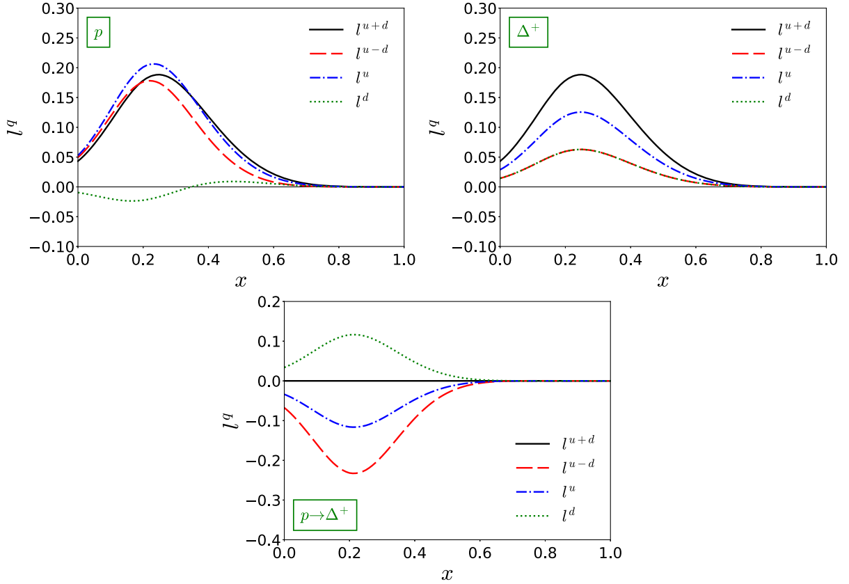
FIG. 2. OAM quark distribution functions for the proton (upper left panel), \Delta^+ baryon (upper right panel), and p \rightarrow \Delta^+ transition (lower panel). The solid (black), dashed (red), dot-dashed (blue), and dotted (green) lines represent the l^{u+d} , l^{u-d} , l^u , and l^d contributions, respectively.
