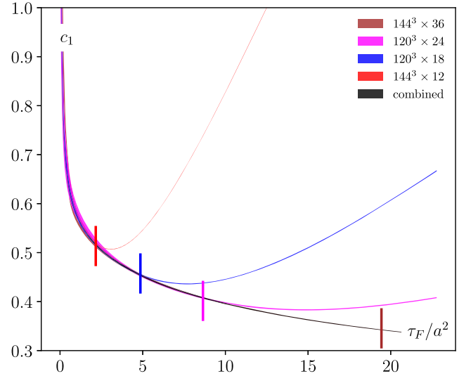
FIG. 1. c_1 measured at several higher temperatures at \beta = 7.544 and their weighted average. The vertical bars indicate the flow depth where each N_\tau choice is expected to become unreliable.
