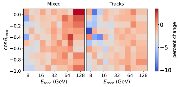
FIG. 32. Ice scattering.
