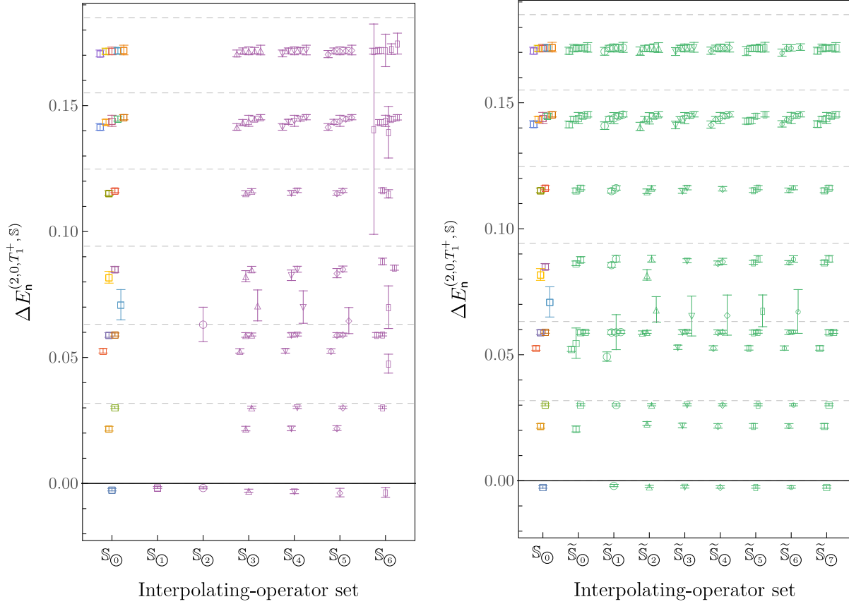
FIG. 26. FV energy shifts obtained using GEVP correlation functions with interpolating-operator set S_{\odot}^{(2,0,T_1^+)} (left column in each panel and corresponding to Figs. 19–21) are compared to results obtained using the interpolating-operator sets defined in Eq. (71) and featured in Fig. 25 (left) as well as the eight other interpolating-operator sets defined in Eq. (72) (right). The color coding for S_{\odot}^{(2,0,T_1^+)} energies follows that in Figs. 19–21, and the dashed lines show noninteracting two-nucleon energies as in Fig. 22.
