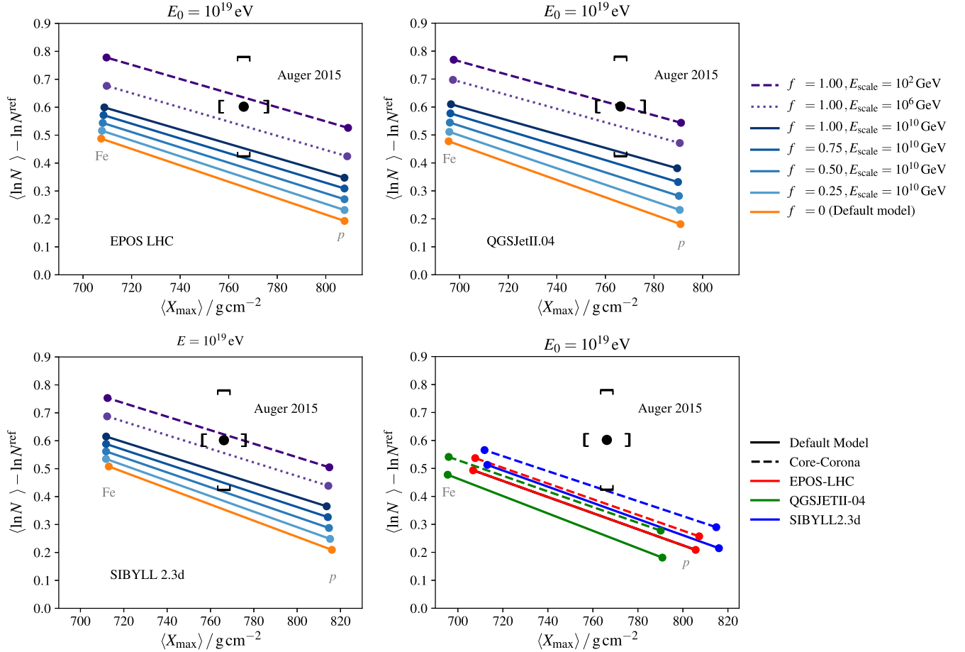
FIG. 6. The impact of different core-corona mixing scenarios on air shower simulations at 10^{19} eV in the X_{\max} - \ln N_{\mu} plane using EPOS LHC (top left), QGSJETII.04 (top right), SIBYLL 2.3d (bottom left), and the ALICE-motivated model corresponding to the shaded area in Fig. 5. The solid lines represent changing the scale f_{\omega} , while the dashed lines also indicate the effect of changing E_{\text{scale}} . The default model corresponds to the corona-only simulations. The datum is from the Pierre Auger Observatory [5]. Each model line represents all values that can be obtained for any mixture of cosmic nuclei from proton (bottom right) to iron (top left). In the bottom-right panel, the full lines are the default model and the dashed line the ALICE-motivated core-corona mixing.
