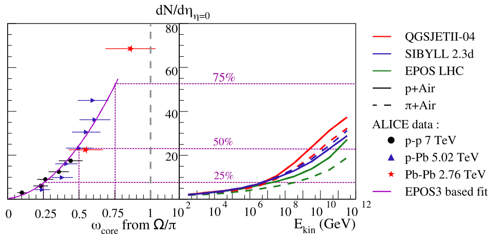
FIG. 4. Energy evolution of particle density at mid-rapidity for proton (solid lines) and pion (dashed lines) interaction with air for different hadronic interaction models (right-hand side) compared to \omega_{\text{core}} as extracted from the \Omega/\pi from [63] (left-hand side). Data points are from ALICE [20] recorded at pseudorapidity |\eta| < 0.5 . See text for details.
