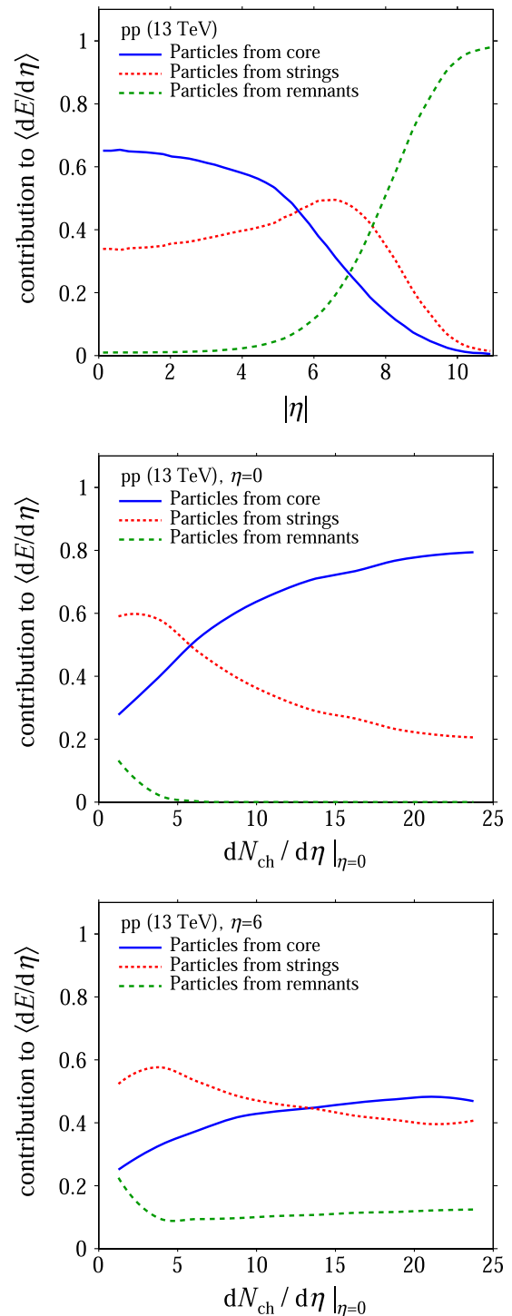
FIG. 2. Fractional contribution of particles originating from different production mechanisms to the total energy density dE/d\eta as predicted by EPOS LHC. The top figure shows the contribution as function of |\eta| ; the middle (bottom) figure shows the contributions at \eta = 0 ( \eta = 6 ) as a function of the charged particle density at \eta = 0 .
