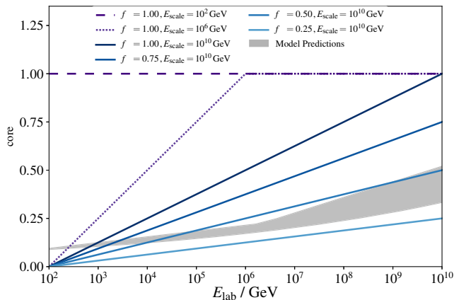
FIG. 5. Different energy evolutions probed for \omega_{\text{core}} . The solid lines represent changing the scale f_\omega of the effect, while the dashed lines also indicate the effect of changing E_{\text{scale}} . The shaded area is based on Fig. 4 motivate by ALICE data and current predictions on particle densities of the EPOS3 model.
