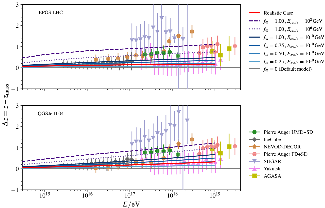
FIG. 7. Evolution of the mass corrected z factor, \Delta z = z - z_{\text{mass}} , as a function of the primary energy. The data are taken from Ref. [9], where the muon content measured by AGASA [91], IceCube [92], KASCADE-Grande [93], NEVOD-DECOR [94,95], Pierre Auger [96,97], SUGAR [98], and Yakutsk [99] are compared. Overlaid are predictions obtained from changing the scale f_\omega (solid lines) and E_{\text{scale}} (dashed and dotted lines) obtained with EPOS LHC (top) and QGSJETII.04 (bottom) air shower simulations.
