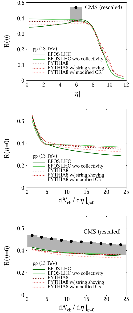
FIG. 3. Ratio of the average electromagnetic to hadronic energy densities R simulated for proton-proton collisions at 13 TeV with EPOS LHC (solid lines) with and without hydrodynamical treatment of the dense core, as well as PYTHIA8 (dashed lines) in the default configuration, with string shoving and with modified color reconnection (CR). The top figure shows R(\eta) as a function of |\eta| , the middle and bottom figure show R evaluated at \eta = 0 and \eta = 6 as a function of the central charged particle multiplicity. The asymmetric uncertainties of the CMS data are a feature of this measurement.
