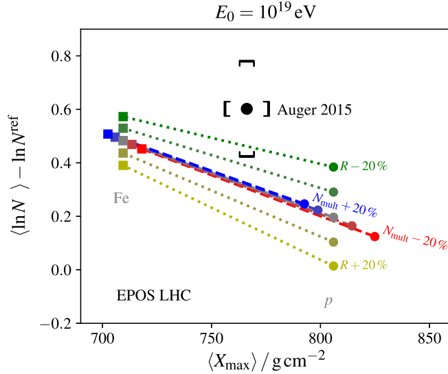
FIG. 1. Impact of the modification scales f_q (in %) of the hadron multiplicity N_{\text{mult}} (dashed lines) and the energy ratio R (dotted lines) in collisions at the LHC energy of \sqrt{s} = 13 TeV on EPOS LHC predictions of the air shower observables X_{\text{max}} and \ln N_{\mu} in 10^{19} eV air showers. The datum is from the Pierre Auger Observatory [5]. The model lines represent all values that can be obtained for any mixture of cosmic nuclei from proton (bottom right) to iron (top left).
