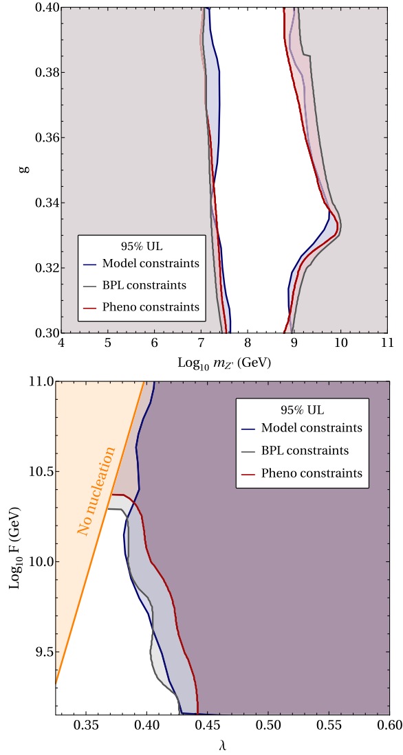
FIG. 4. Comparison of the constraints on the parameter space (m_Z, g) for Model I (top panel) and on (\lambda, F) for Model II (bottom panel) obtained by constraining the model parameters directly as in Fig. 3 (blue line), with those obtained by adopting the BPL model as given in Fig. 1 (gray line), and those adopting the phenomenological model in Fig. 2 (red line).
