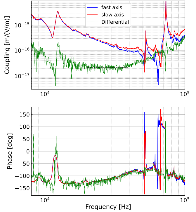
FIG. 10. Calibrated transfer functions. The black dashed line shows the fitted result between 20–40 kHz.
