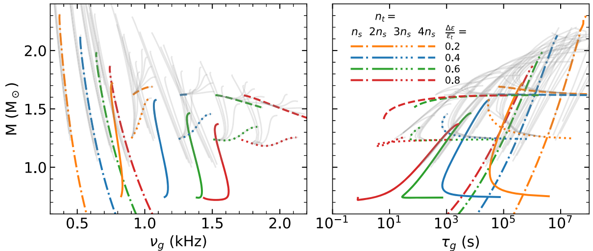
FIG. 12. The left (right) panel shows the g -mode frequency (damping time) versus mass for hybrid NSs modeled with \chi EFT and the CSS parametrization. Colored lines correspond to cases with c_s^2 = 1/3 while gray lines show results with higher values of c_s^2 .
