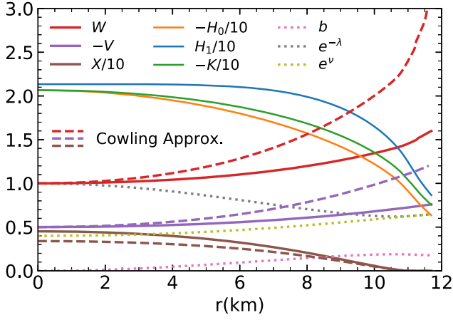
FIG. 14. Metric perturbation amplitudes, fluid perturbation amplitudes for nonradial oscillations with \ell = 2 with (dashed curves) and without (solid curves) the Cowling approximation, and static metric functions (dotted curves) inside a 1.4M_{\odot} NS computed with the Sly4 EOS [85]. H_0 , H_1 and K are in units of \epsilon_s = 152.26 \text{ MeV fm}^{-3} , X is in units of \epsilon_s^2 , and W , V , \nu and \lambda are dimensionless. Only real parts of the perturbation amplitudes are plotted.
