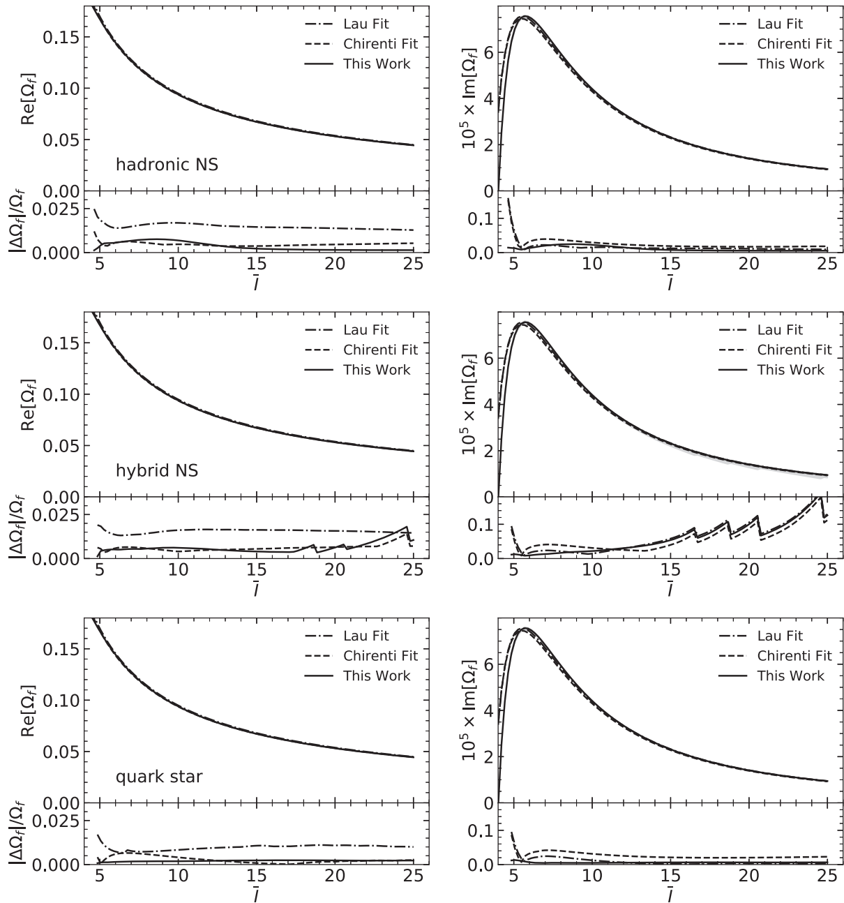
FIG. 7. The same as Fig. 6 except for the \Omega_f - \bar{l} universal relation. “This work” refers to Eq. (18) and other fits are due to Refs. [7] (Lau) and [10] (Chirenti) are shown.
