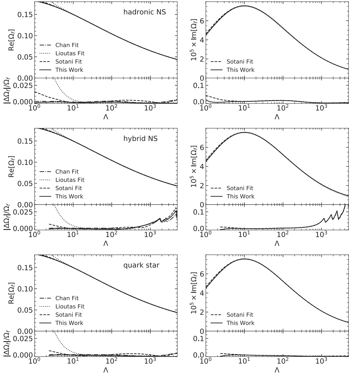
FIG. 8. The same as Fig. 6 but for the \Omega_f - \Lambda universal relation. “This work” refers to Eq. (19) and other fits due to Refs. [9] (Chan), [11] (Lioutas), and [79] (Sotani) are shown.
