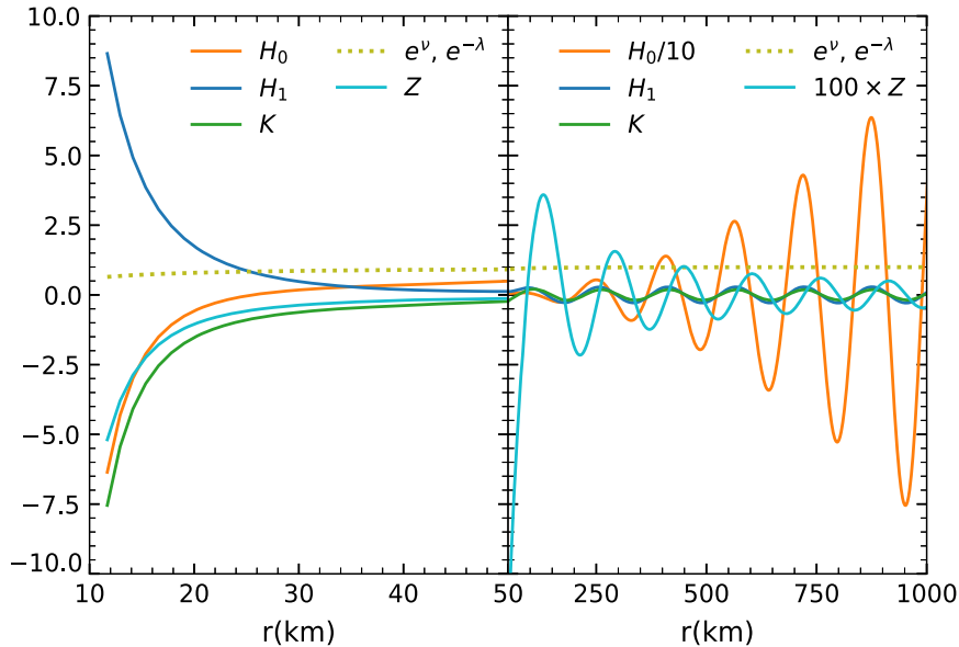
FIG. 15. The same as Fig. 14 except outside the 1.4M_\odot SLy4 EOS NS. Note the change of scale at r = 50 \text{ km} .
