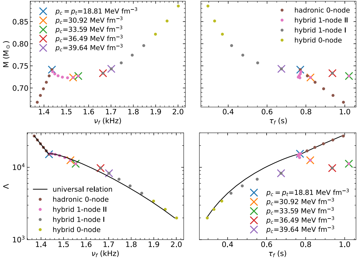
FIG. 10. f -mode frequency and damping time for hybrid NSs with small quark cores as functions of mass and tidal deformability. Brown and yellow dots represent stars with normal f -modes having no radial nodes, while pink and gray dots represent stars with the special 1-mode behavior. The colored crosses correspond to 5 configurations displayed in Fig. 9. In the tidal deformability plots, the universal relations from Eq. (19) are shown.
