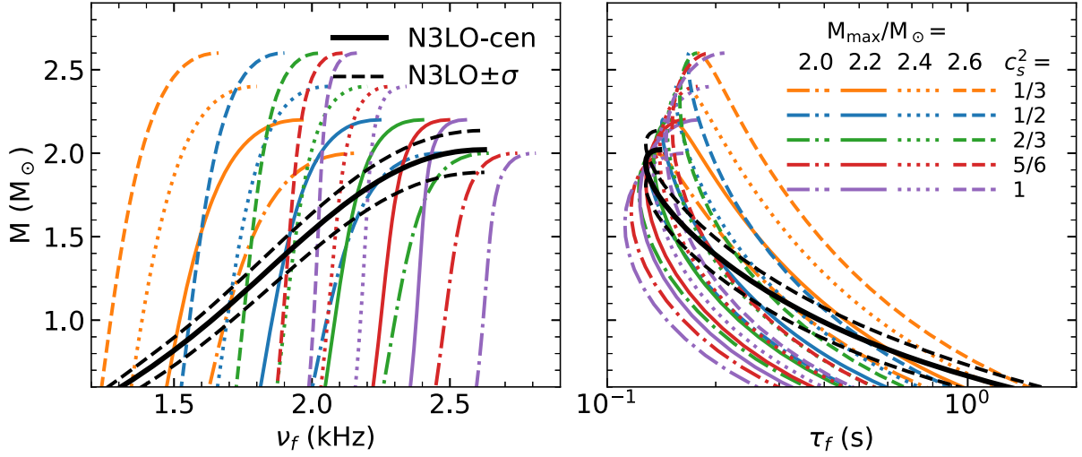
FIG. 2. The left (right) panel shows the f -mode frequency (damping time) as a function of M for pure quark stars with the CSS parametrization (colored curves) compared to hadronic stars employing the N3LO-cen EOS and its one-sigma uncertainty bounds (black curves).
