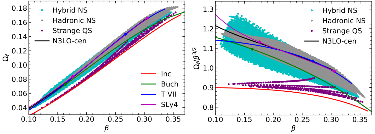
FIG. 4. The dimensionless f -mode frequency \Omega_f as a function of stellar compactness \beta for parametrized hadronic, hybrid and quark matter stars constrained by causality and M_{\max} \geq 2M_{\odot} . General relativistic results for the analytic EOSs and the SLy4 and N3LO-cen hadronic EOSs are shown for comparison.
