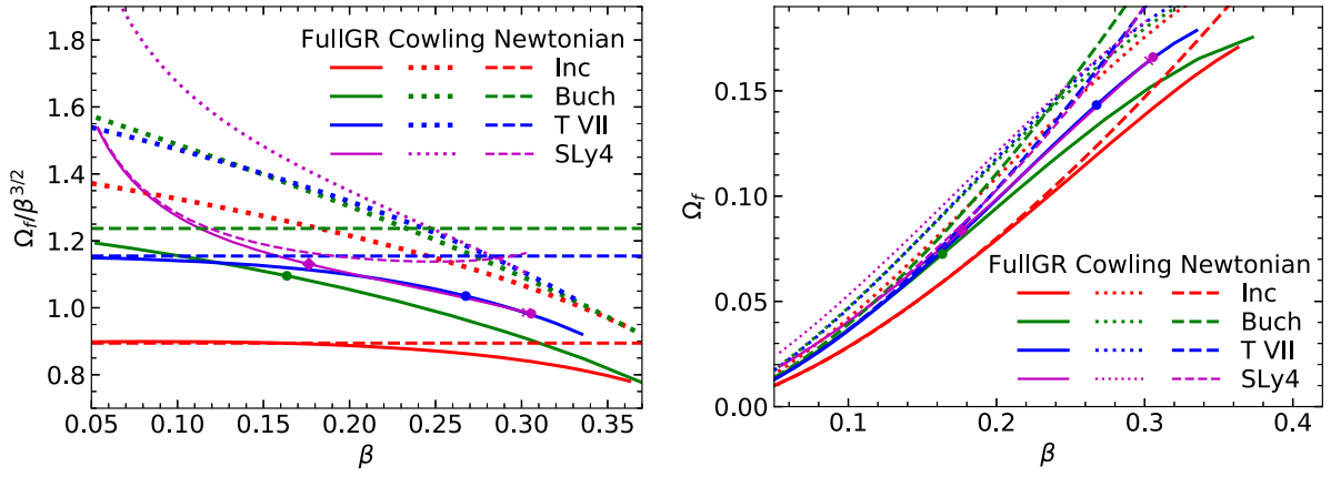
FIG. 1. Dimensionless f -mode frequency versus compactness \beta for the SLy4 and three analytic EOSs. Solid lines show the result of linear perturbation theory in general relativity, dashed lines show the Newtonian result (i.e., the Kelvin-mode frequency), and dotted lines show results assuming the Cowling approximation. Dots on the SLy4, T VII and Buch solid lines indicate \beta values where causality c_s = 1 occurs; the diamond on the SLy4 solid lines indicates the 1.4M_\odot configuration.
