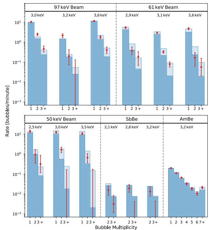
FIG. 13. Comparison between the measured bubble rate (in bubbles per minutes) and fit of the data. The red points are the experimental data points with Feldman-Cousins 1\sigma confidence intervals as error bars on the Poisson mean in each bin [28]. The blue histograms are the result of the MCNP/GEANT4 simulations convolved with the bubble efficiency curves fit to the data; the empty blue bars represent the \pm 1\sigma error window of the fit.
