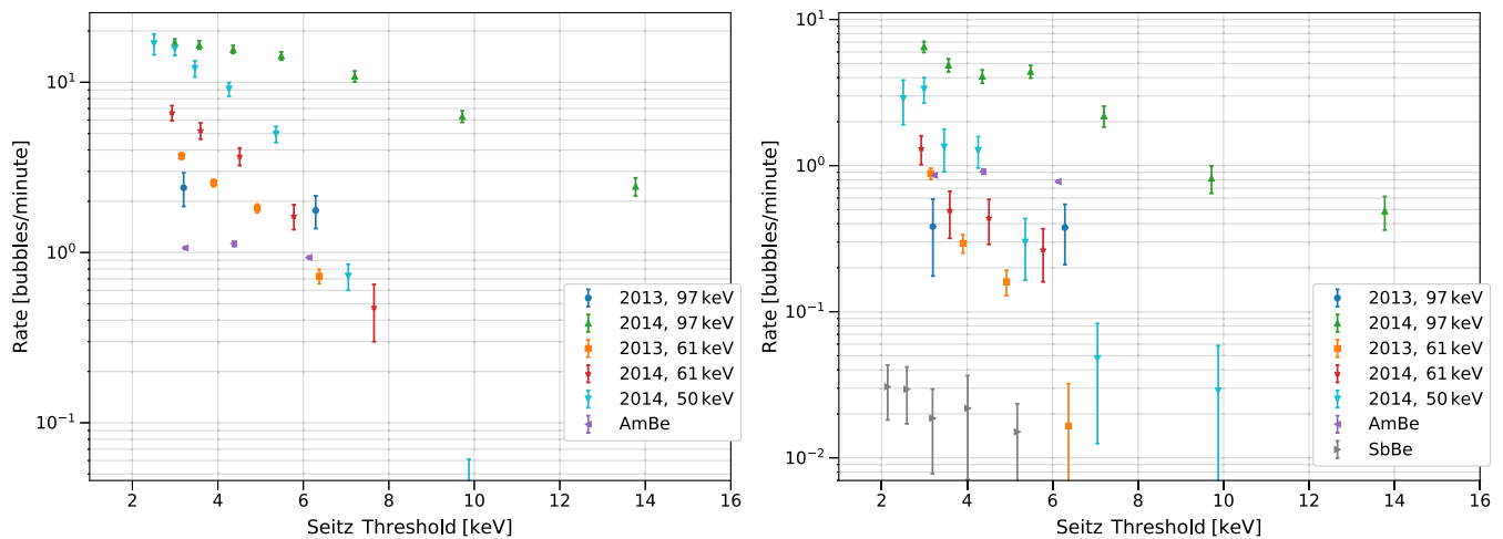
FIG. 7. Background-subtracted measured rates of events with one or more bubble (left) and with two or more bubbles (right), in units of bubbles per minute (counting each bubble separately in multibubble events). Error bars show statistical uncertainty only. The background rates subtracted were approximately 0.2 single bubbles/minute for beam data (much less for higher multiplicity events), 0.004 2 bubble events per minute for the SbBe data, and 0 for the AmBe data (below the sensitivity of the background measurement). Data at Seitz thresholds greater than 3.6 keV are not included in the full analysis, but the trends with Seitz threshold illustrate the relative sensitivity of each dataset to the underlying nuclear recoil detection threshold.
