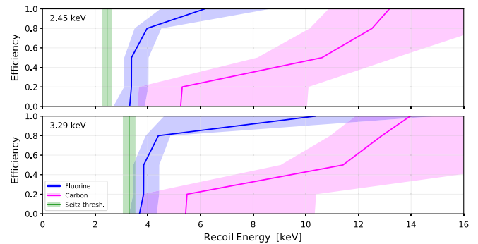
FIG. 12. Best-fit and 1\sigma error bands for the nucleation efficiency curves of fluorine (blue) and carbon (magenta), at the thresholds used in the PICO-60 WIMP search [5]. Error bands indicate the 1\sigma range of each knot position, so that every efficiency curve within 1\sigma of the best fit falls in the shaded area (but not every curve falling in the shaded area is within 1\sigma of the best fit). The corresponding Seitz thresholds are shown as a vertical green line, with the green band indicating the systematic threshold uncertainties described in Table IV.
