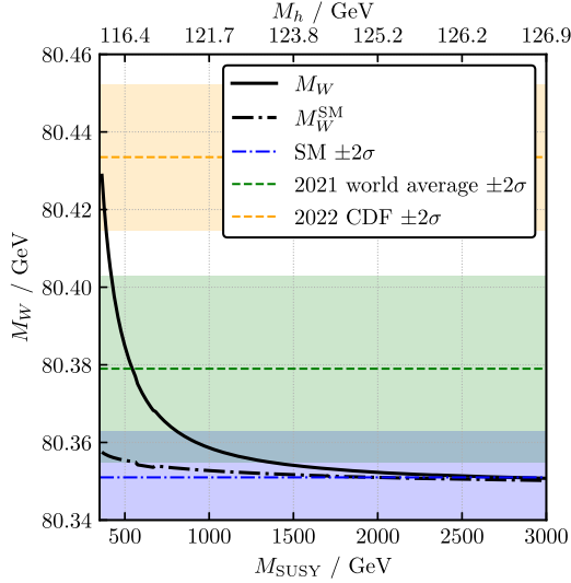
FIG. 1. Prediction of M_W in the MSSM as a function of the common supersymmetry scale M_{\text{SUSY}} (black solid line). The black dash-dotted line shows the SM prediction using the \overline{\text{MS}} fit formula from Ref. [2] for the corresponding value of the Higgs pole mass M_h (top axis). The blue dash-dotted line shows the SM prediction M_W^{\text{SM}} = (80.351 \pm 0.006) GeV for the fixed value of the Higgs pole mass M_h = 125.25 GeV, including its uncertainty. The green dashed line shows the 2021 world average experimental value M_W^{2021} = (80.379 \pm 0.012) GeV including its uncertainty. The orange dashed line shows the CDF value M_W^{\text{CDF}} = (80.4335 \pm 0.0094) GeV including its uncertainty.
