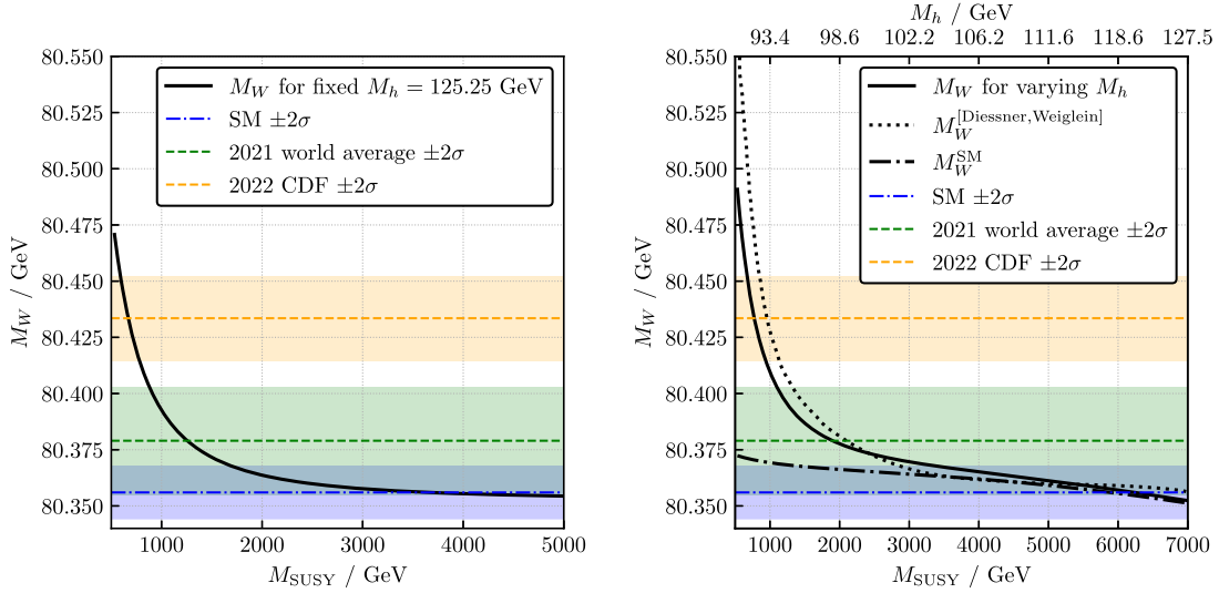
FIG. 3. Prediction of M_W in the MRSSM as a function of the common supersymmetry scale M_{\text{SUSY}} (black solid line), for parameter values as given in Eq. (18) and below. In the left panel the Higgs pole mass that is used to calculate M_W^{\text{SM}} is fixed to M_h = 125.25 GeV. In the right panel the Higgs pole mass as predicted by the MRSSM is used to calculate M_W^{\text{SM}} . The black dash-dotted line shows the SM prediction using the \overline{\text{MS}} fit formula from Ref. [2] for the corresponding value of the Higgs pole mass M_h (top axis). The black dotted line shows the prediction from Ref. [30]. The blue dash-dotted line shows the SM prediction M_W^{\text{SM}} = (80.354 \pm 0.006) GeV for the fixed value of the Higgs pole mass M_h = 125.25 GeV, including its uncertainty. The green dashed line shows the 2021 world average experimental value M_W^{2021} = (80.379 \pm 0.012) GeV including its uncertainty. The orange dashed line shows the CDF value M_W^{\text{CDF}} = (80.4335 \pm 0.0094) GeV including its uncertainty.
