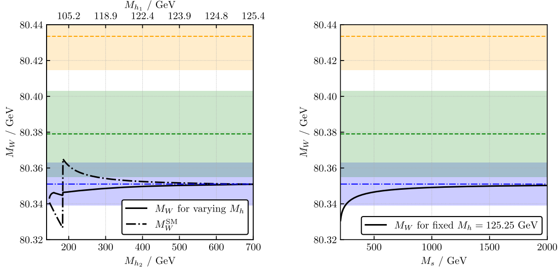
FIG. 2. Prediction of M_W in the Scalar Singlet Model with a \mathbb{Z}_2 symmetry. The blue, green and orange lines and regions are as in Fig. 1. In the left panel, the parameter set (15a) is used. As in Fig. 1, the solid black lines indicate the prediction of M_W where the Higgs mass has been allowed to vary, and the black dash-dotted line shows the SM prediction using Eq. (45) from Ref. [2]. The light and heavier Higgs masses are shown on the top and bottom axes, respectively. The right panel uses the parameter set from (15b) and shows the prediction of M_W for a Higgs boson pole mass fixed to M_h = 125.25 GeV, as a function of the scalar mass M_s , which is shown on the bottom axis.
