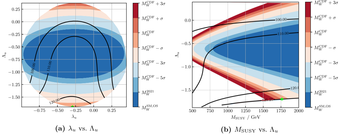
FIG. 4. Prediction of the W boson pole mass M_W and contours for the Higgs boson pole mass M_h in the MRSSM around the point \tan\beta \approx 24.7 , \Lambda_d \approx -1.59 , \Lambda_u = -1.70 , \lambda_d \approx 2.18 , \lambda_u \approx -0.293 , and M_{\text{SUSY}} \approx 1763 GeV (marked with a \star ). The color contours label landmark M_W values in terms of the number of standard deviations from M_W^{\text{CDF}} , or in the case of medium and dark blue bands, the 2021 world average and the SM on shell prediction, respectively. As such the value for M_W varies a lot among the colored regions.
