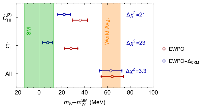
FIG. 1. The resulting values of \Delta m_W = m_W - m_W^{\text{SM}} when turning on \hat{C}_{Hl}^{(3)} , \hat{C}_{ll} , and all Wilson coefficients that are probed by EWPO. The red bars indicated the predicted \Delta m_W from the EWPO fit, while the blue bars show the resulting \Delta m_W after inclusion of \Delta_{\text{CKM}} . The shown values of \Delta\chi^2 denote the differences in the minimum \chi^2 between the blue and red points. The SM prediction and world average, taken from Ref. [18], are depicted by the green and orange bands, respectively.
