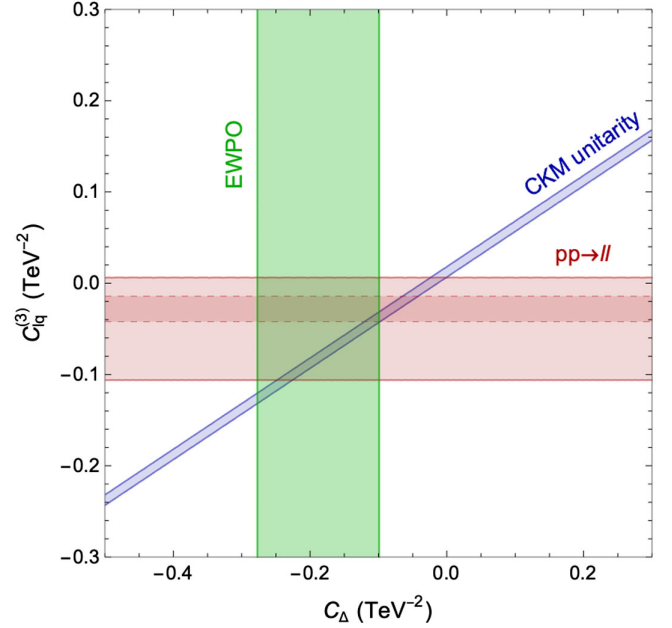
FIG. 2. The 1\sigma constraints from EWPO in green, a global (single-coupling) analysis of LHC measurements in (dashed) red, and low-energy beta decays in blue.
