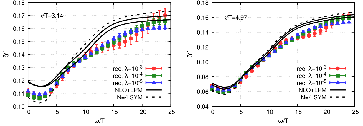
FIG. 3. Comparison of filtered, rescaled, transverse channel spectral functions obtained using the continuum lattice data (with colors) and the perturbative spectral function (continuous, black), as well as the \mathcal{N} = 4 SYM theory (dashed, black) for k/T \approx 3.14 and k/T \approx 4.97 (left and right panels, respectively). The renormalization scale is set to \mu = 2\pi T or \mu = 3\pi T when using the NLO + LPM spectral function, which results in two curves. The renormalization scales 2\pi T and 3\pi T correspond to \alpha_s \approx 0.31 and \alpha_s \approx 0.25 , respectively. Errors are only statistical.
