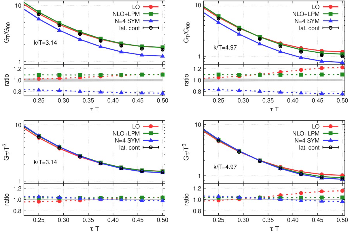
FIG. 2. Top panels: Comparison of the G_T/G_{00} correlators for k/T = \pi and k/T \approx 4.97 . The bottom insets show the various correlators normalized by the continuum-extrapolated lattice-QCD correlator. The NLO + LPM result is obtained by using \alpha_s = 0.25 . Bottom panels: Comparison of G_T/T^3 . We set N_c = 3 to obtain the SYM theory result.
