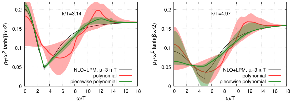
FIG. 8. Reconstructed spectral functions using the NLO + LPM weak coupling G_T/G_{00} mock correlator as an input.
