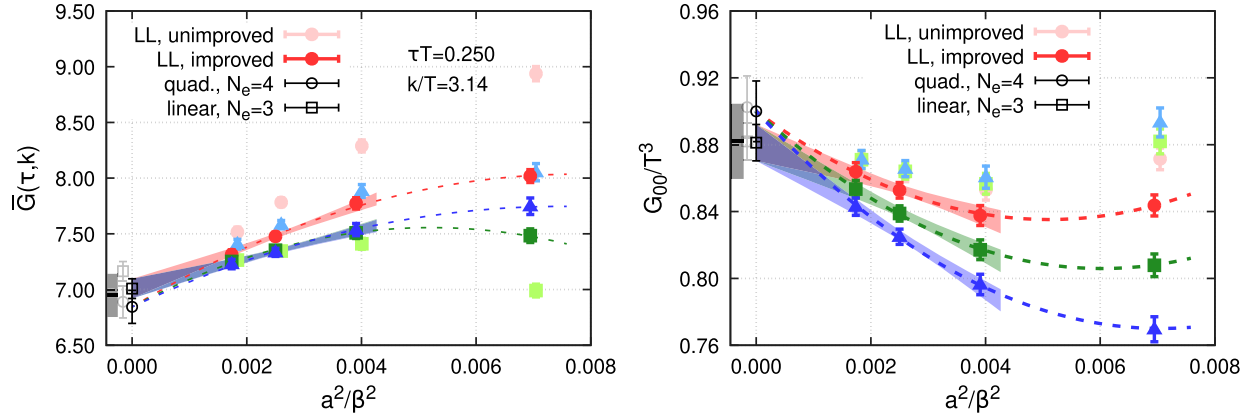
FIG. 1. Left : Simultaneous continuum extrapolation at \tau T = 0.25 of the local-local (LL), local-conserved (LC), and conserved-conserved (CC) tree-level improved correlators plotted with red circles, blue triangles, and green squares, respectively. The unimproved correlator values are shown with fainter symbols. The colored bands show the linear fit using the three finest lattice spacings and all discretizations, while the dashed lines illustrate the quadratic fit using all data points. The results of the linear (quadratic) extrapolations are shown as empty squares (circles). The fainter, shifted, gray symbols show the continuum values obtained using the unimproved correlators. The leftmost gray band represents our final continuum estimate, including its systematic error. Right : Simultaneous continuum extrapolation of the isovector charge-charge correlator required to compute the static susceptibility. The color code is the same as in the left panel.
