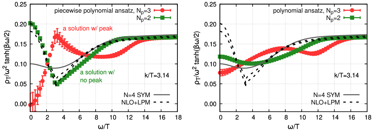
FIG. 5. Left : Representative fit results using the piecewise polynomial Ansatz with two ( N_p = 2 ) or three fit parameters ( N_p = 3 ) at k/T = \pi . For comparison, the transverse channel spectral function in the weak coupling NLO + LPM theory, as well as in the strongly coupled SYM theory are also included. Right : Representative fit results using the polynomial Ansatz .
