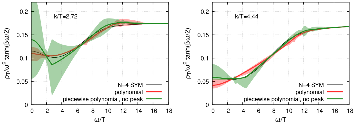
FIG. 12. Reconstructed spectral functions using the strongly coupled \mathcal{N} = 4 SYM theory mock correlator, G_T/T^3 , as an input.
