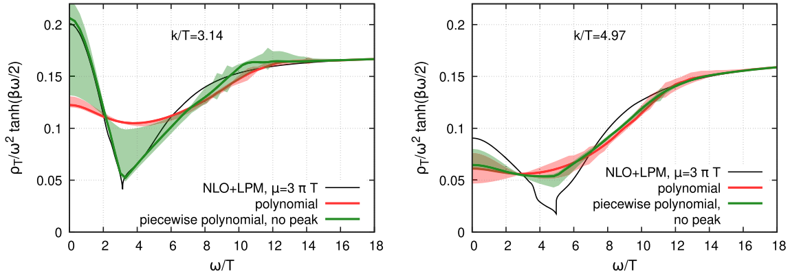
FIG. 9. Reconstructed spectral functions using the NLO + LPM weak coupling G_T/T^3 mock correlator as an input.
