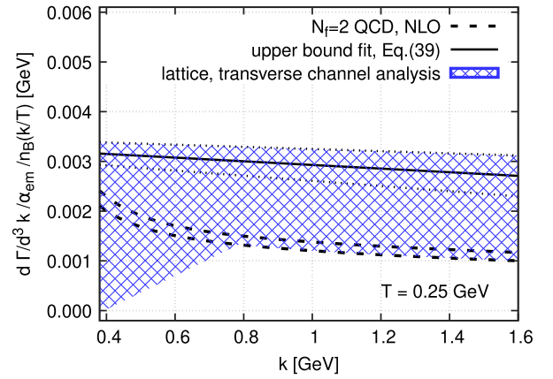
FIG. 7. The photon rate per unit volume of the QGP at T \simeq 250 MeV (hatched band). The Bose factor n_B = 1/(e^{k/T} - 1) has been divided out. The upper bound parametrization derived from the D_{\text{eff}} results of the polynomial Ansatz is shown as a solid line. The full leading-order results [11] obtained by setting \alpha_s \simeq 0.25 or 0.31 are shown for comparison. Including corrections from interactions with soft gluons, one can get a 20% increase at \alpha_s \simeq 0.3 for the perturbative result [12].
