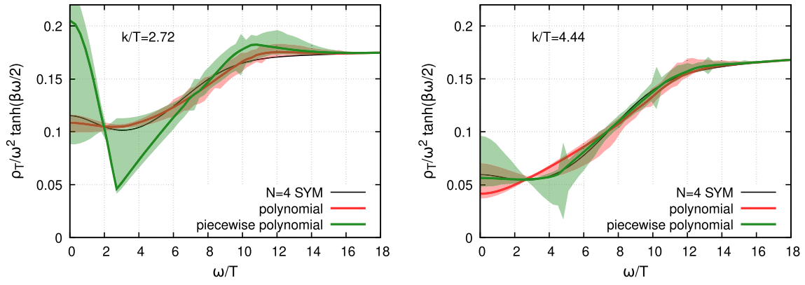
FIG. 11. Reconstructed spectral functions using the strongly coupled \mathcal{N} = 4 SYM theory mock correlator, G_T/G_{00} , as an input.
