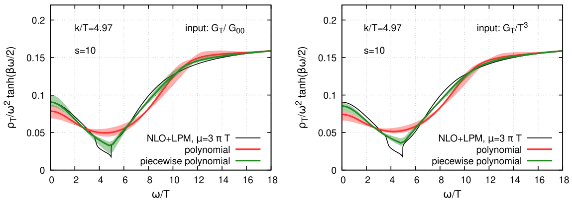
FIG. 10. Reconstructed spectral functions using the NLO + LPM correlator G_T/G_{00} (left), or G_T/T^3 (right) as an input. The covariance matrix elements have been decreased by a factor of s^2 = 100 . Having such small errors, the piecewise polynomial Ansatz could better approximate the dip.
