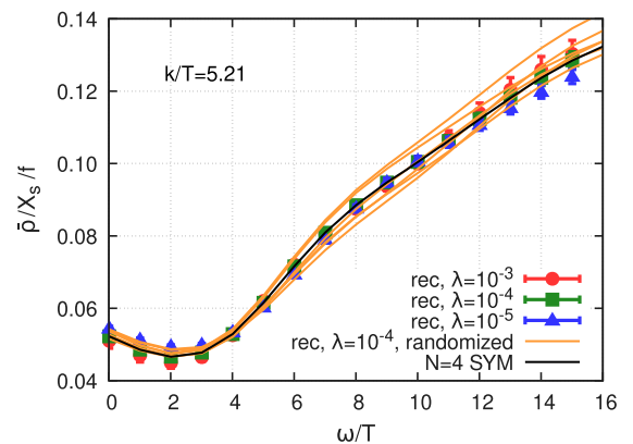
FIG. 13. Reconstructed, filtered spectral functions using the \mathcal{N} = 4 SYM mock correlator, \bar{G}_T^{(\text{mock})} = G_T^{(\text{mock})}/G_{00}^{(\text{mock})} , as an input. The results obtained with the help of the six randomized mock correlators are shown in orange without including the statistical errors. These errors are comparable to the errors of the reconstructed \hat{\rho} using the exact model data.
