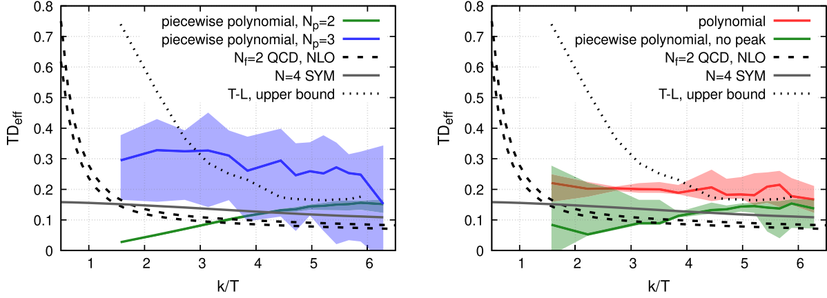
FIG. 6. Results for the effective diffusion coefficient, TD_{\text{eff}} , defined in Eq. (10). Left: Separate analyses of fit results obtained with N_p = 2 and N_p = 3 using the piecewise polynomial Ansatz [Eq. (37)]. Right: Imposing the constraint of Eq. (38) at 1 standard deviation to the fit results obtained with the piecewise polynomial Ansatz. The results obtained by using the polynomial Ansatz [Eq. (36)] are displayed in red. Analytical results from perturbative QCD [11] using \alpha_s \simeq 0.25 or 0.31 (dashed lines) and from the strongly coupled \mathcal{N} = 4 SYM theory (gray line) [40] are also included, as well as an upper bound obtained from the analysis of the T – L channel (dotted line) [24]. We use the value \chi_s/T^2 = 0.88(2) to obtain TD_{\text{eff}} from the lattice data, but the free susceptibility to obtain TD_{\text{eff}} from the N_f = 2 weak coupling photon rate.
