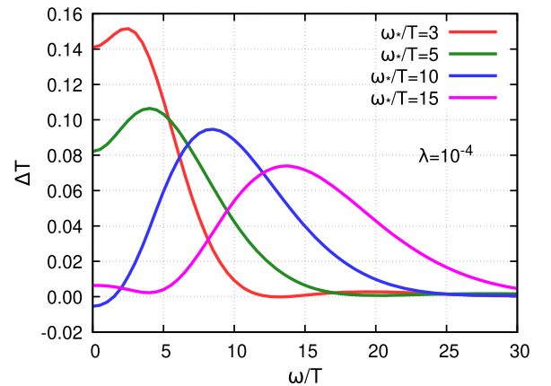
FIG. 4. Resolution functions for k/T \approx 3.14 , \lambda = 10^{-4} for different values of \omega_*/T .
