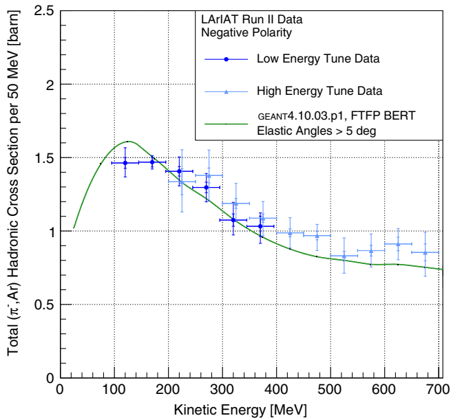
FIG. 15. \pi^- , Ar total hadronic cross section for scattering angles greater than 5^\circ measured in the LArIAT low energy and high energy tune run II data samples. The GEANT4 prediction for the total hadronic cross section for inelastic scattering and elastic scattering angles greater than 5^\circ is displayed in green.
