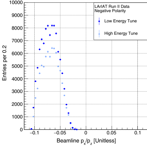
FIG. 5. Distribution of the p_x to p_z momentum ratio for electrons, muons, and pions in the LArIAT beamline for run II negative polarity data, low energy tune in dark blue, high energy tune in light blue. The x component of the particles' momentum is small, since particles are mostly directed in the z direction. The p_x/p_z shows an offset of the mean relative to the beam axis due to the action of the bending magnets.
