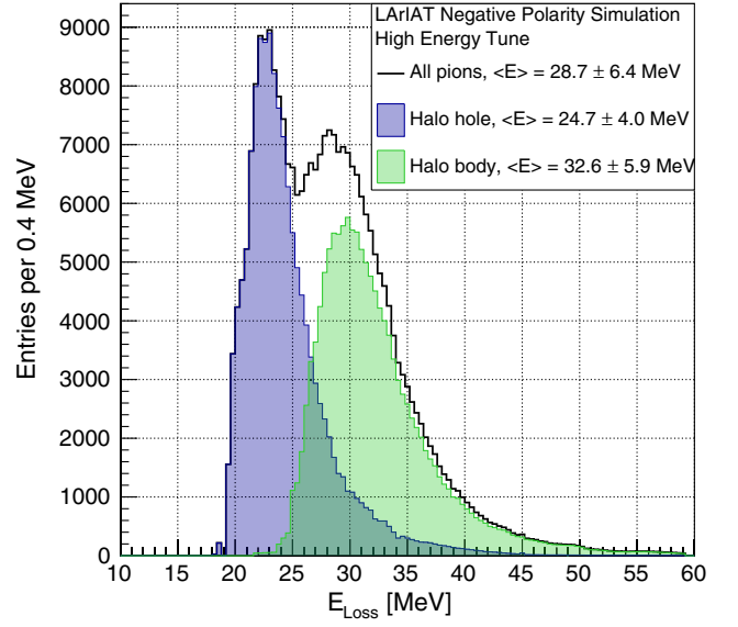
FIG. 12. True energy loss between the fourth wire chamber and the LArTPC front face according to the simulation of negative polarity events for the high energy tune. Two populations are visible, depending on the amount of material traversed by the beamline pion. The HALO scintillator paddle—a rectangular piece with a central hole—is responsible for the double-peaked distribution. The distribution for the pions traveling through the central hole (missing the scintillator material) is shaded in purple, and the distribution for the pions hitting the HALO body is shaded green, the sum of these distributions is indicated by the black histogram.
