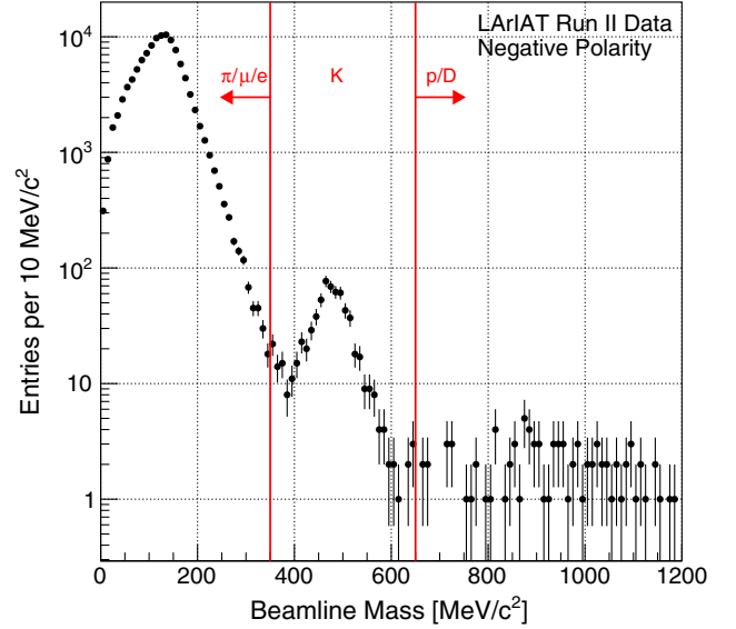
FIG. 7. Distribution of the beamline mass as calculated according to Eq. (3) for the run II events reconstructed in the beamline, for negative polarity runs. The classification of the events into \pi^-/\mu^-/e^- , K^- , or antiproton is based on these distributions, whose selection values are represented by the vertical red lines.
