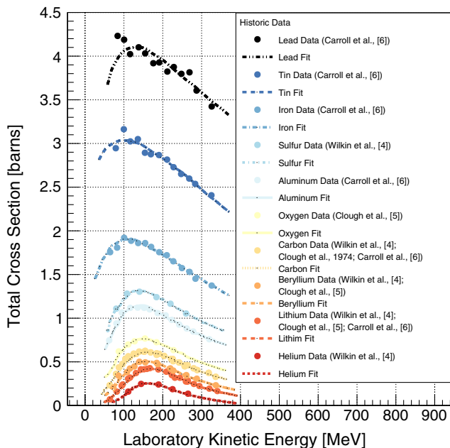
FIG. 1. Historical positive pion scattering data for different light and heavy nuclei, reproduced from Ref. [6].
