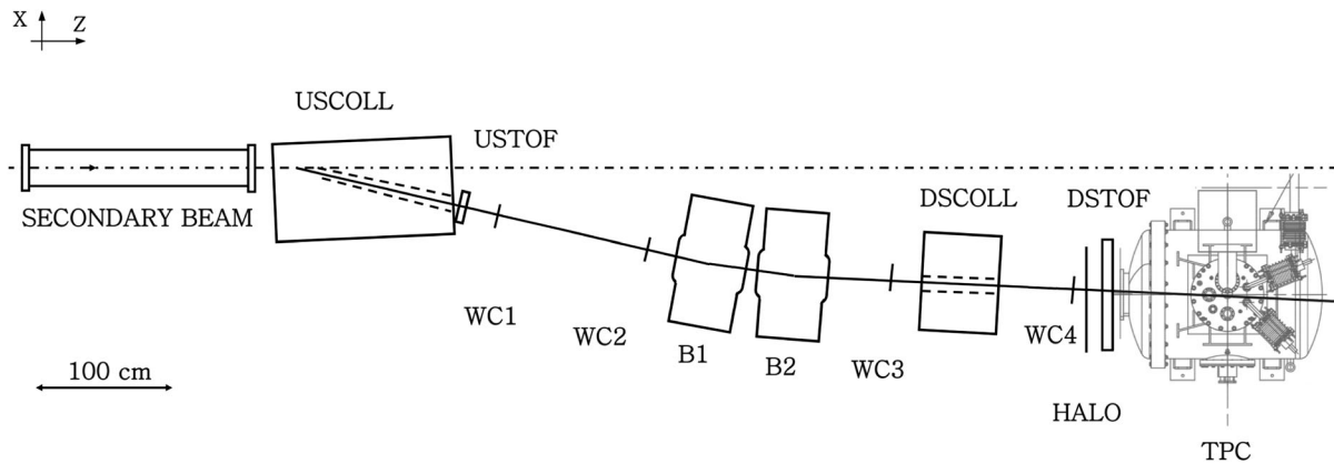
FIG. 3. Bird's-eye view of the LArIAT tertiary beamline. USCOLL and DSCOLL represent the upstream and downstream collimators respectively; B1 and B2 represent the bending magnets; WC1, WC2, WC3, and WC4 are the multiwire proportional chambers; USTOF and DSTOF represent the upstream and downstream time-of-flight scintillators; HALO represents a scintillator paddle with a central hole to enable vetoes of particles with trajectories incompatible with the beamline path; TPC shows the technical drawing of the cryostat which surrounds the liquid argon time projection chamber.
