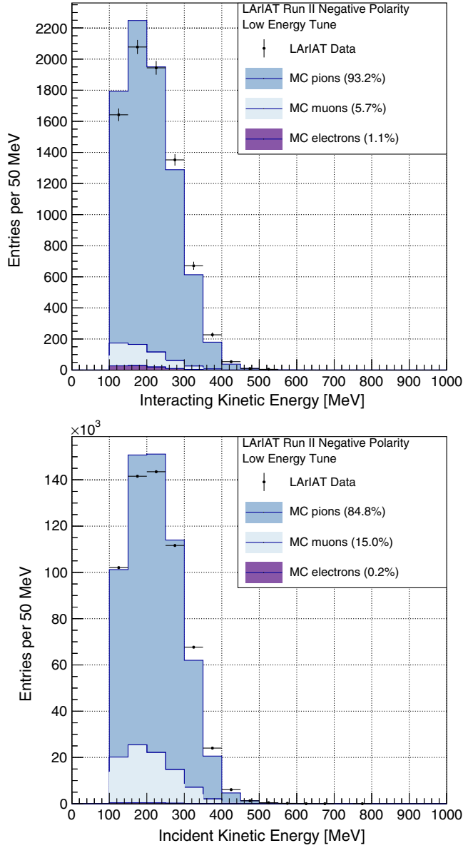
FIG. 13. Interacting and incident fluxes for the low energy tune. The simulated stacked contributions for pions (dark blue), muons (light blue) and electrons (purple) are normalized to the number of pion candidates selected in low energy tune data.
