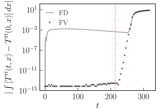
FIG. 1. Discrete conservation of T^{tt} across the spatial domain for a simulation starting from Gaussian initial data (48) with \eta_0 = 0.2 for the finite volume scheme presented here (FV) as well as the semi-finite-difference scheme of [36] (FD). As expected, the finite volume scheme conserves T^{tt} up to machine precision \sim 10^{-15} , until the fluid pulse reaches the boundary at the time marked by the light red dotted line. The semi-finite-difference scheme of [36] conserves T^{tt} only up to the level of truncation error, which in this case is \sim 10^{-3} .
