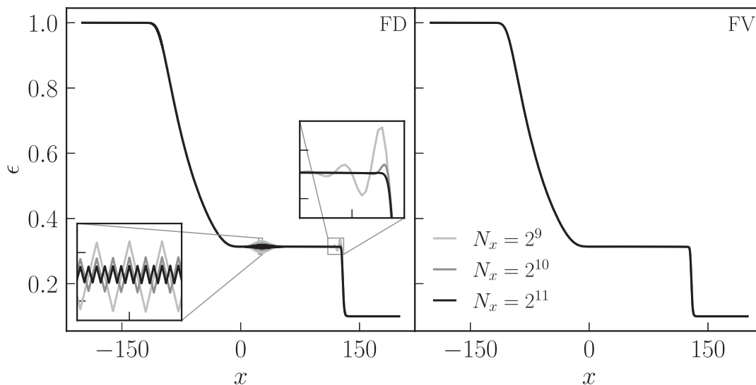
FIG. 4. Comparison of solutions for \epsilon starting from shock tube initial data (51) at three successive resolutions for the semi-finite-difference scheme of [36] (left, FD) versus the finite volume scheme presented here (right, FV) at t \sim 43 for \eta_0 = 0.2 . The FD scheme has oscillations near the shock front which quickly converge away with resolution, as well as grid-scale “sawtooth” oscillations that developed early on near the origin (the t = 0 location of the shock front) and do not converge away as rapidly with resolution. These features do not appear in the figures of [36] because the discontinuities there are smaller in amplitude, leading to oscillations small enough to be tamed by applying Kreiss-Oliger dissipation; said dissipation is not strong enough to remove the oscillations for the initial data (51), and we choose not to apply artificial dissipation in either scheme throughout this work. The FV solutions are free of noticeable oscillations, and the N_x = 2^9, 2^{10}, 2^{11} curves all overlap at the resolution of the plot.
