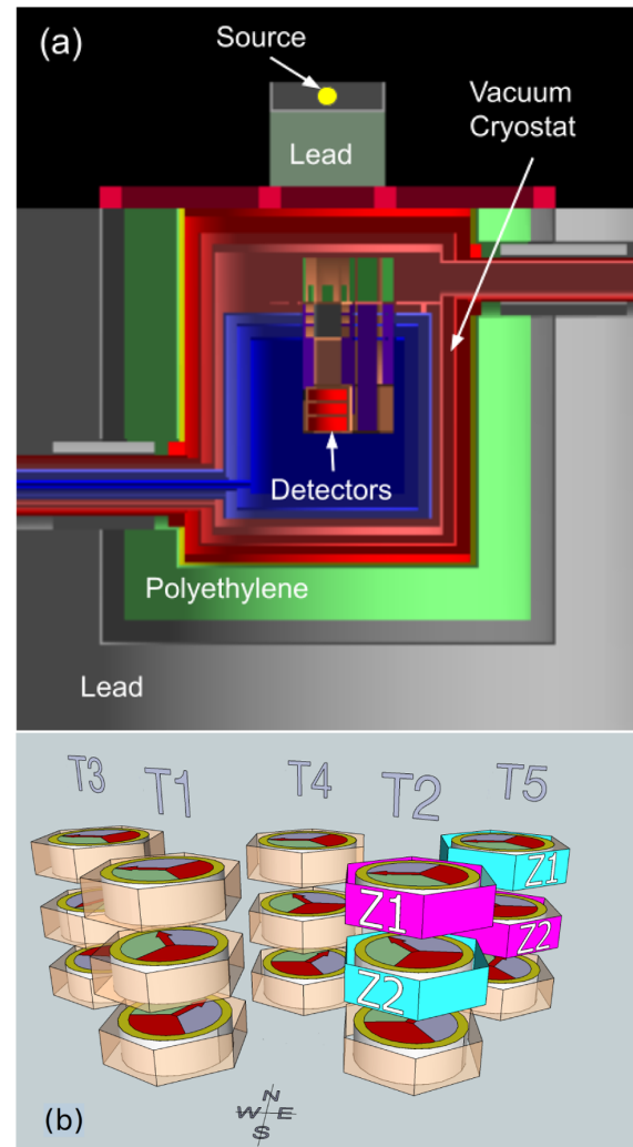
FIG. 2. (a) The experimental setup with the shielding configuration. Lead was used to shield against gammas. Polyethylene shielding was required for the dark matter configuration, and only the top portion was removed from the experiment in order to perform the photo-neutron calibration. (b) Detectors were arranged into five towers with three detectors in each tower. Each face of the detectors had four phonon channels. The phonon channel layout is indicated by the different colours on the upper face of the detector. The photo-neutron source was placed above and between towers T2 and T5. The T2Z1 and T5Z2 detectors used in this analysis have been highlighted in pink. The detectors T2Z2 and T5Z1, highlighted in blue, were used for a systematic study of the event rate due to the position of the source over the two towers.
