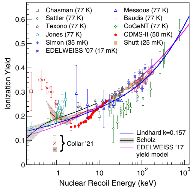
FIG. 1. Literature data on ionization yield measurements as a function of recoil energy in germanium [8,11–25]. Measurements by Shutt, Simon, EDELWEISS, and CDMS-II are in the mK temperature range, while all others are at 77 K. The CDMS II yield measurements are from a single detector [15] that is similar to the averaged yield over all detectors. However, variation across individual detectors was more than the statistical uncertainty of the measurement shown here [16]. EDELWEISS has reported two measurements: (i) discrete yield measurements using a ^{252}\text{Cf} neutron source [19], and (ii) continuous measurement using an ^{241}\text{Am}^9\text{Be} neutron source fitted by a power law function considered as their yield model [24]. The work by Collar et al. reports three different approaches to measuring ionization yield in germanium: (i) using photoneutrons from an ^{88}\text{Y}^9\text{Be} source indicated by the red band, (ii) using nuclear recoils from thermal neutron capture indicated by the red hollow square marker, and (iii) using an iron-filtered low energy neutron beam [25]. The prediction by Lindhard et al. [6,26] is also shown for comparison.
