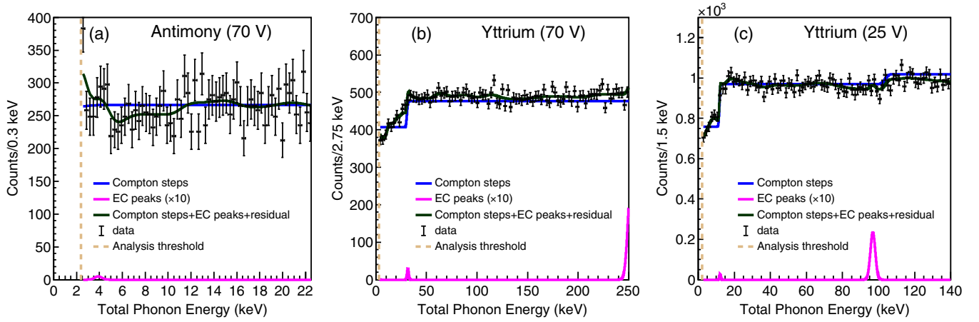
FIG. 6. Neutron-OFF energy spectrum for the three data sets: (a) ^{124}\text{Sb}^9\text{Be} with T5Z2 biased at 70 V, (b) ^{88}\text{Y}^9\text{Be} with T5Z2 biased at 70 V, and (c) ^{88}\text{Y}^9\text{Be} with T2Z1 biased at 25 V. The contribution from each component in the background model is shown. The contribution of the electron capture peaks have been scaled up by a factor of 10 for better visualization.
