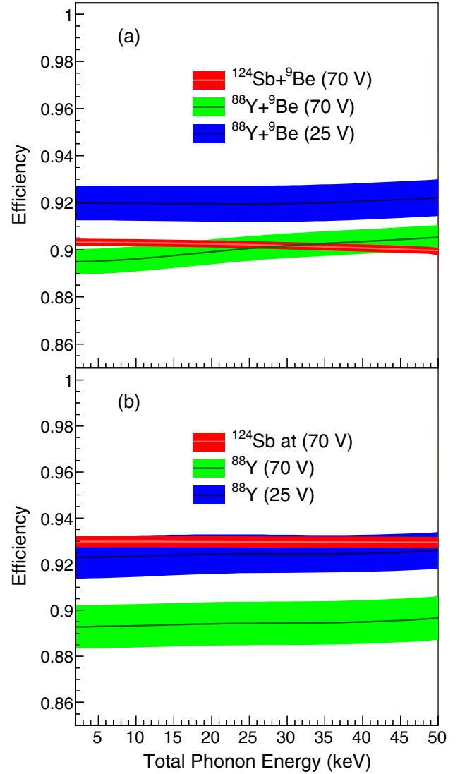
FIG. 3. Combined and smoothed cut efficiency as a function of energy above the analysis threshold for each data set with a 1\sigma uncertainty. (a) With the Be wafer, i.e., neutron-ON, and (b) without the Be wafer, i.e., neutron-OFF.
