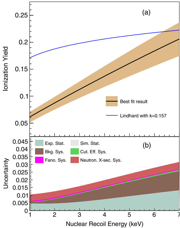
FIG. 8. (a) The ionization yield with 1\sigma uncertainty from the best fit values of the two-component k -parameter Lindhard model as a function of the nuclear recoil energy in germanium. The blue line shows the standard Lindhard model with k = 0.157 . (b) The contribution of various sources of statistical and systematic uncertainties to the ionization yield in germanium. The lower limit of the x axis represents the analysis threshold converted to recoil energy using the best-fit value.
