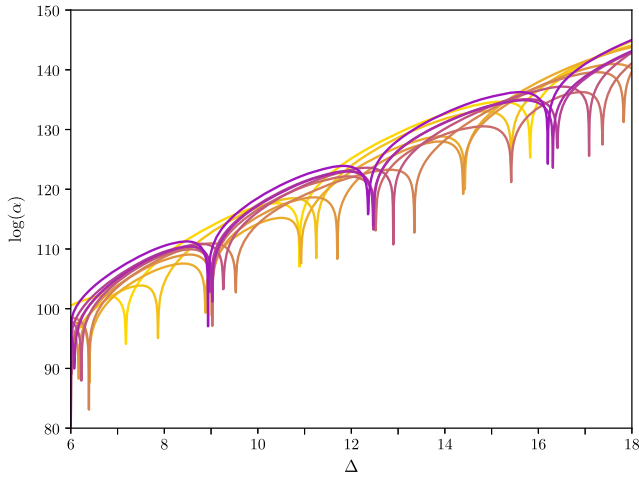
(a) \mathfrak{f} = \mathfrak{so}_{20}
