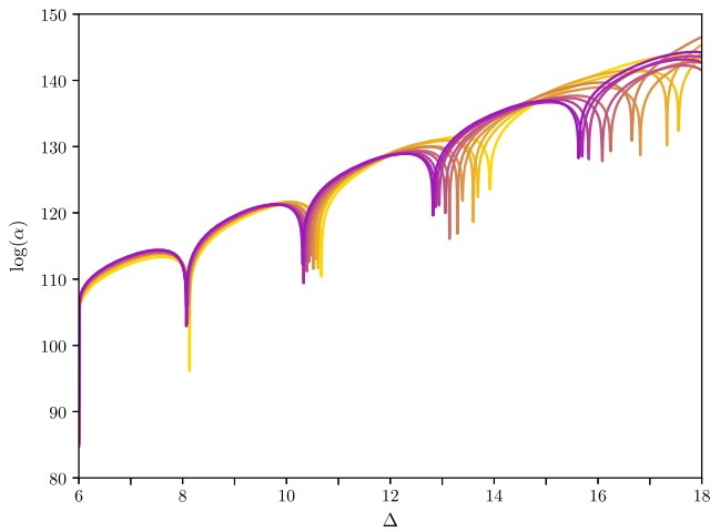
(c) \mathbf{f} = \mathbf{s0}_{200}
