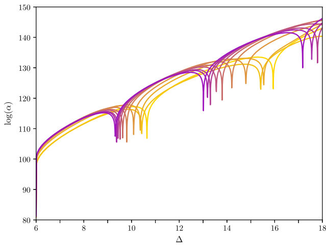
(b) \mathfrak{f} = \mathfrak{so}_{40}
