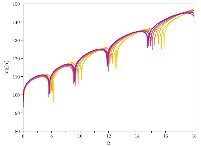
(c) \mathbf{f} = \mathbf{s0}_{200}
