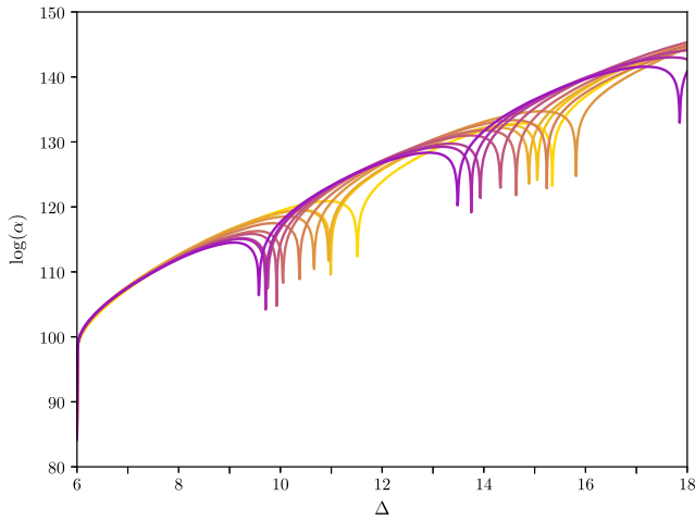
(c) \mathfrak{f} = \mathfrak{so}_{200}
