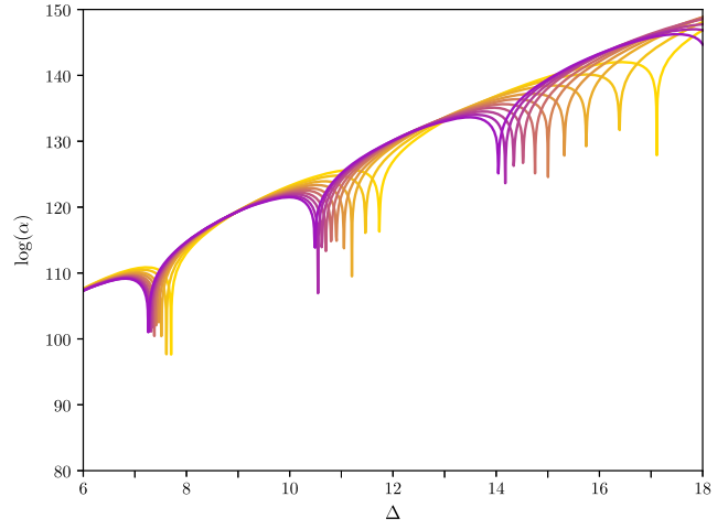
(a) \mathfrak{f} = \mathfrak{so}_{20}
