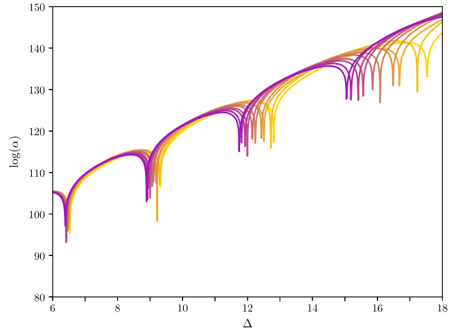
(a) \mathbf{f} = \mathbf{s0}_{20}
