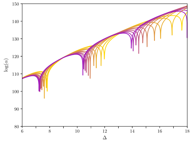
(b) \mathfrak{f} = \mathfrak{so}_{40}
