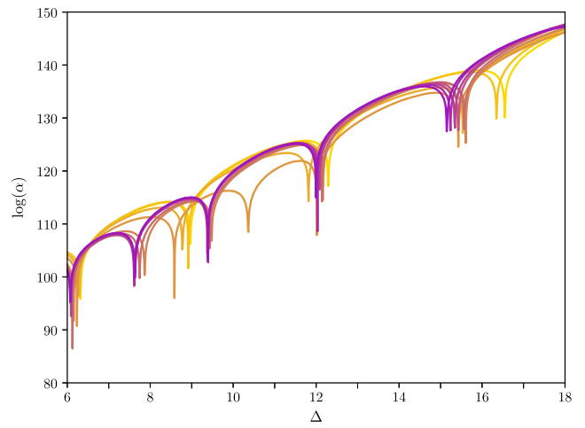
(b) \mathbf{f} = \mathbf{s0}_{40}
