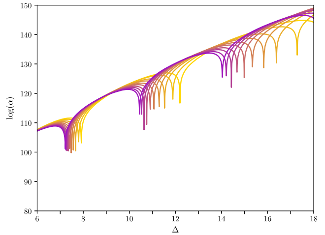
(c) \mathfrak{f} = \mathfrak{so}_{200}
