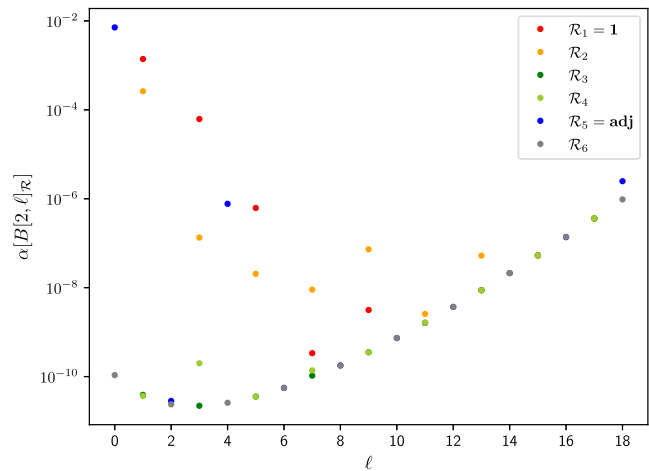
FIG. 8. Value of the functional with \Lambda = 49 and \mathfrak{f} = \mathfrak{so}_{200} applied to \mathcal{B}[2, \ell]_{\mathcal{R}} multiplets. Representations not satisfying the constraint in Eq. (18) do not appear in the OPE from the outset.
