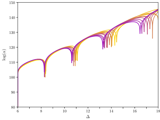
(a) \mathbf{f} = \mathbf{s0}_{20}
