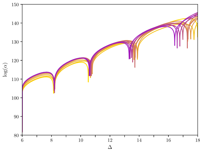
(b) \mathbf{f} = \mathbf{s0}_{40}
