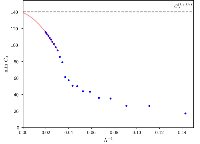
FIG. 2. Bootstrap lower bounds on C_J for theories with flavor symmetry \mathfrak{so}_{20} . The red lines correspond to quadratic interpolations for points with either \Lambda \geq 33 or \Lambda \geq 35 . The derivative cutoffs are \Lambda = 7, 9, \dots, 49, 51 .
