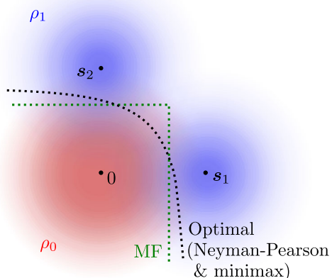
FIG. 5. Suboptimality of matched filtering under the minimax framework.
