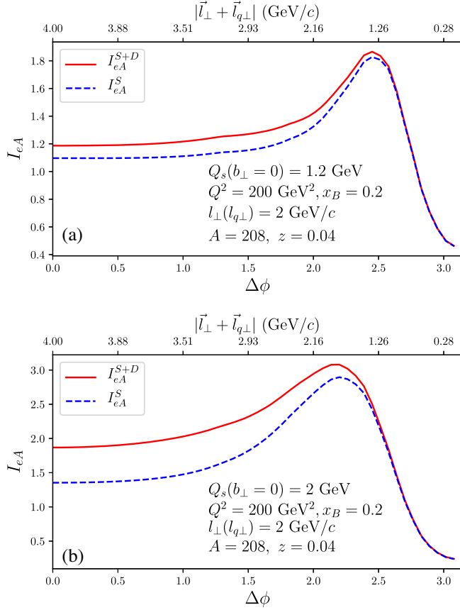
FIG. 10. The total nuclear modification factor I_{eA}^{S+D}(l_{\perp}, l_{q\perp} = l_{\perp}, \Delta\phi, z) and that from only single scattering I_{eA}^S(l_{\perp}, l_{q\perp} = l_{\perp}, \Delta\phi, z) as a function of the azimuthal angle \Delta\phi or the transverse momentum imbalance |\vec{l}_{\perp} + \vec{l}_{q\perp}| in e + \text{Pb} DIS with x_B = 0.2 and Q^2 = 200 \text{ GeV}^2 for (a) Q_s(0_{\perp}) = 1.2 \text{ GeV} and (b) Q_s(0_{\perp}) = 2 \text{ GeV} .
