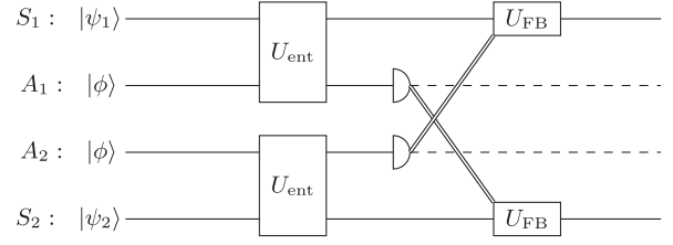
FIG. 7. Adversarial measurement-and-feedback gravity, following [45]. The figure is taken from [7].
