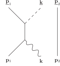
FIG. 10. Disconnected diagram for Eq. (B22).
