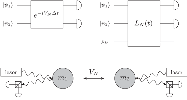
FIG. 1. Top: two masses m_1, m_2 are prepared in an initial product state, interact gravitationally for a time \Delta t , and are read out to check for entanglement. Left: unitary Newtonian interaction. Right: an effective Newtonian channel L_N emerges from environmental interactions. Bottom: minimal experimental realization with free-falling masses. The Newton interaction would squeeze the relative position x_- while preserving total momentum p_+ , leading to a violation of the Duan inequality [26,27] for separable states \langle \Delta x_-^2 \Delta p_+^2 \rangle \geq \hbar^2 . This can be read out with local interferometers.
