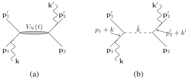
FIG. 3. Scattering amplitude for the 3 \rightarrow 3 process with external photons, in the same notation as Fig. 2. (a) Nonrelativistic amplitude; (b) its relativistic extension.
