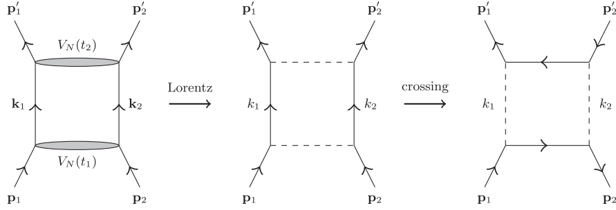
FIG. 12. Basic procedure to compute the elastic \chi\bar{\chi} scattering amplitude. The left diagram represents the nonrelativistic \chi\chi \rightarrow \chi\chi scattering amplitude, computed to second order in perturbation theory. Its relativistic extension is depicted in the middle panel. Finally, by crossing symmetry, the same mathematical expression can be used to compute the \chi\bar{\chi} \rightarrow \chi\bar{\chi} amplitude to the same order, depicted in the third panel.
