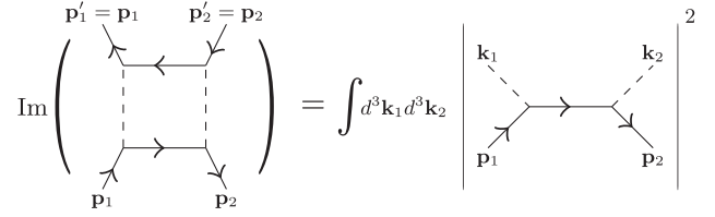
FIG. 13. Forward \chi\bar{\chi} scattering at second order in the gravitational interaction. The imaginary part of the forward amplitude has a branch cut singularity, which precisely equals the total cross section for the process \chi\bar{\chi} \rightarrow gravitons.
