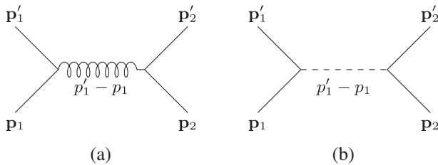
FIG. 5. Some tree-level scattering processes which can reproduce the Newton potential operator: (a) Standard spin-2 graviton exchange; (b) exchange of a spin-0 “scalar graviton”.
