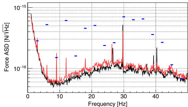
FIG. 2. Amplitude spectral density of the z component of the force on a 7.56 \mu\text{m} diameter MS. The black (red) curve shows actual data with the AS stationary (scanning along y at 3 \text{ Hz} with 202 \mu\text{m} peak-to-peak amplitude). The blue bars show a comparison to an expected MS response produced by the potential described by Eq. (1) with \alpha = 10^{10} and \lambda = 10 \mu\text{m} . The data displayed here is the average of 100 distinct 10 \text{ s} integrations.
