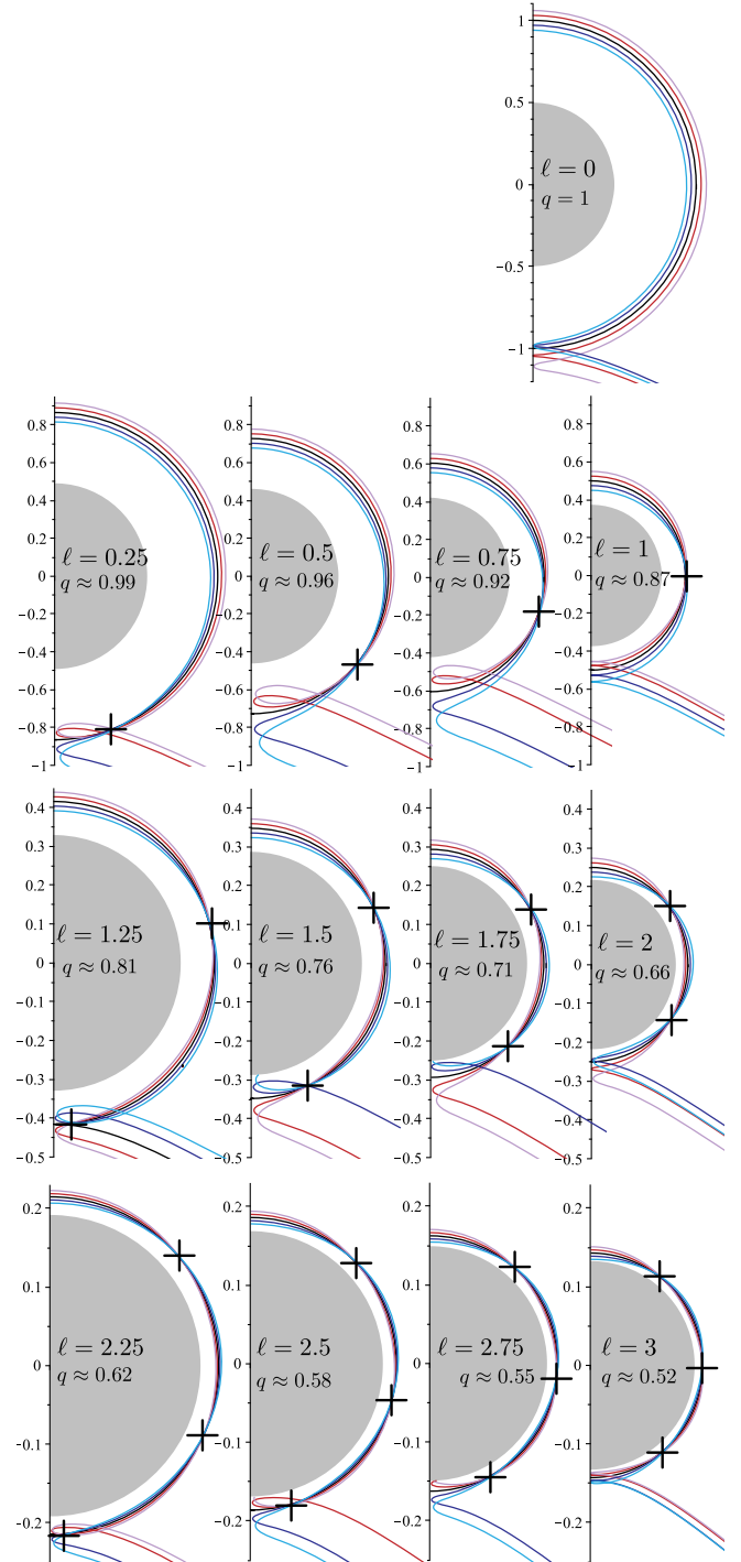
FIG. 9. Inner spherically symmetric MOTS from the Reissner-Nordström spacetime. For a given \ell \in \mathbb{R}^+ , Q = qM for q defined by (110). Thus the m = 0 version of the stability operator has zero negative eigenvalues in the first row, one in the second, two in the third and three in the fourth. The correspondence between the stability operator and deviation equation can then be clearly seen in the number of intersections (again marked with +s) between the nearby MOTSodesics and the inner horizon. The gray circle indicates the region not covered by the Painlevé-Gullstrand coordinates. Note that some MOTSodesics are lost into that region.
