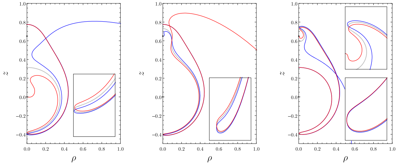
FIG. 10. Nearby MOTSodesics for three of the new MOTSs presented in Fig. 4. In each case, the gray curve corresponds to the MOTS, while the red curve originates slightly inside the MOTS and the blue curve slightly outside. For the MOTS shown here, we have determined that the stability operator has 1, 2 and 2 negative eigenvalues, respectively. We can see that this corresponds also to the number of intersections of nearby MOTSodesics. The insets show a zoomed-in view near the intersections.
