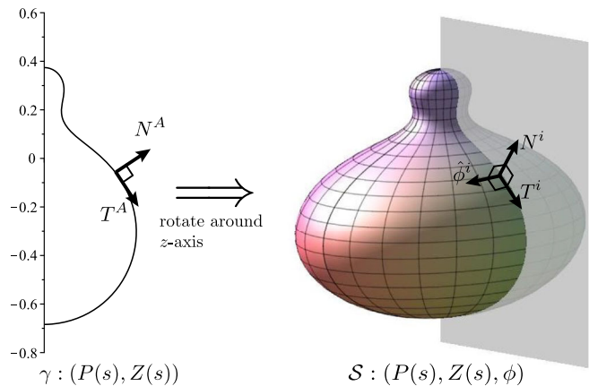
FIG. 1. A curve \gamma that rotates into a surface \mathcal{S} . In the text we see how \Theta_{\pm} = 0 \Leftrightarrow k_N \pm k_u = 0 gives rise to second order equations of motion for \gamma in the (\rho, z) plane. The two-dimensional tangent vector T^A and normal vector N^A to \gamma push-forward to become three-dimensional vectors T^i and N^i .
