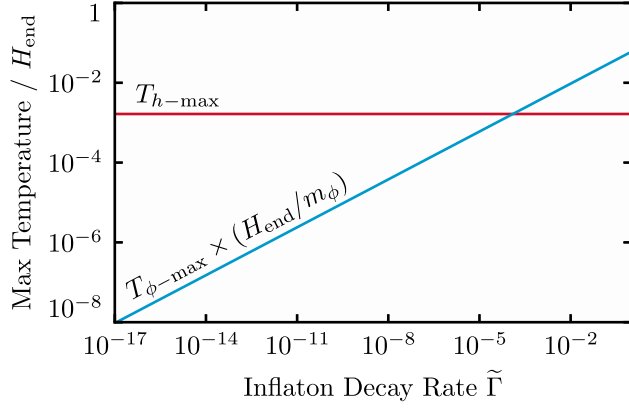
FIG. 4. The maximum temperature during reheating as a function of the inflaton decay rate \tilde{\Gamma} . The Higgs decays to an effectively thermal population at a temperature T_{h\text{-max}} [red, (36)], which dominates over the contribution to the thermal plasma from the inflaton's thermal decay products T_{\phi\text{-max}} [blue, (57)] when \tilde{\Gamma} \lesssim 10^{-4} for H_{\text{end}} \sim m_{\phi} . For further discussion see Sec. IV.
