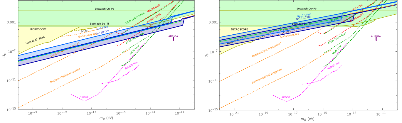
FIG. 4. d_e vs m_\phi for N = 6 (left) and N = 10 (right). Light ( M = 1 TeV) and dark ( M = 10 TeV) blue bands represent a region where no more than 90% of random initial conditions result in either \rho_\phi > \rho_{DM} or \rho_\phi < \rho_{DM} . The green line within the dark blue band is a semianalytic approximation valid in the regime \eta \ll 10^{-4} and the orange line is a semianalytic approximation in the regime \eta \gtrsim 1 , both drawn only for M = 10 TeV. Explicit expressions for both lines were given in Eq. (50) (green) and Eq. (54) (orange). The green band gives current constraints from equivalence principle experiments [43–45], the yellow band presents the current constraints from atomic clock experiments [42,47] while dashed lines give potential reach of the future proposed experiments [39,50–52].
