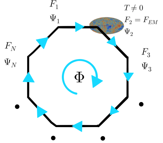
FIG. 1. An illustration of the \mathbb{Z}_N model is shown. There are N copies of the Standard Model and N copies of a heavy hypercharged vectorlike fermion \Psi that are cyclically exchanged under the \mathbb{Z}_N symmetry. A complex scalar \Phi transforms linearly under the \mathbb{Z}_N and has a Yukawa coupling to the fermions \Psi_k .
