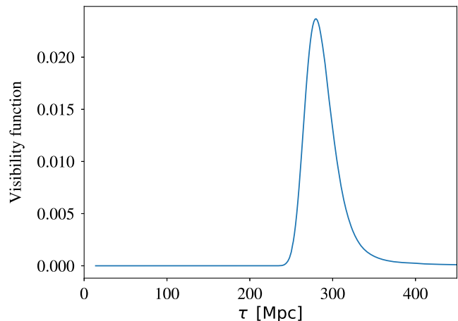
FIG. 2. The CMB visibility function \kappa(\tau_0, \tau) as a function of conformal time. It is shown to indicate the range of conformal times, peaked at \tau \simeq 280 Mpc, that which contribute to the observed CMB power spectra from recombination.
